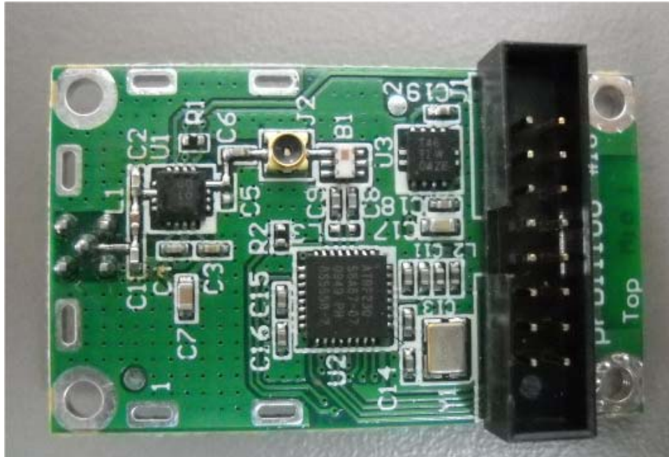
Photograph No.3 LD module bottom view without shielding
