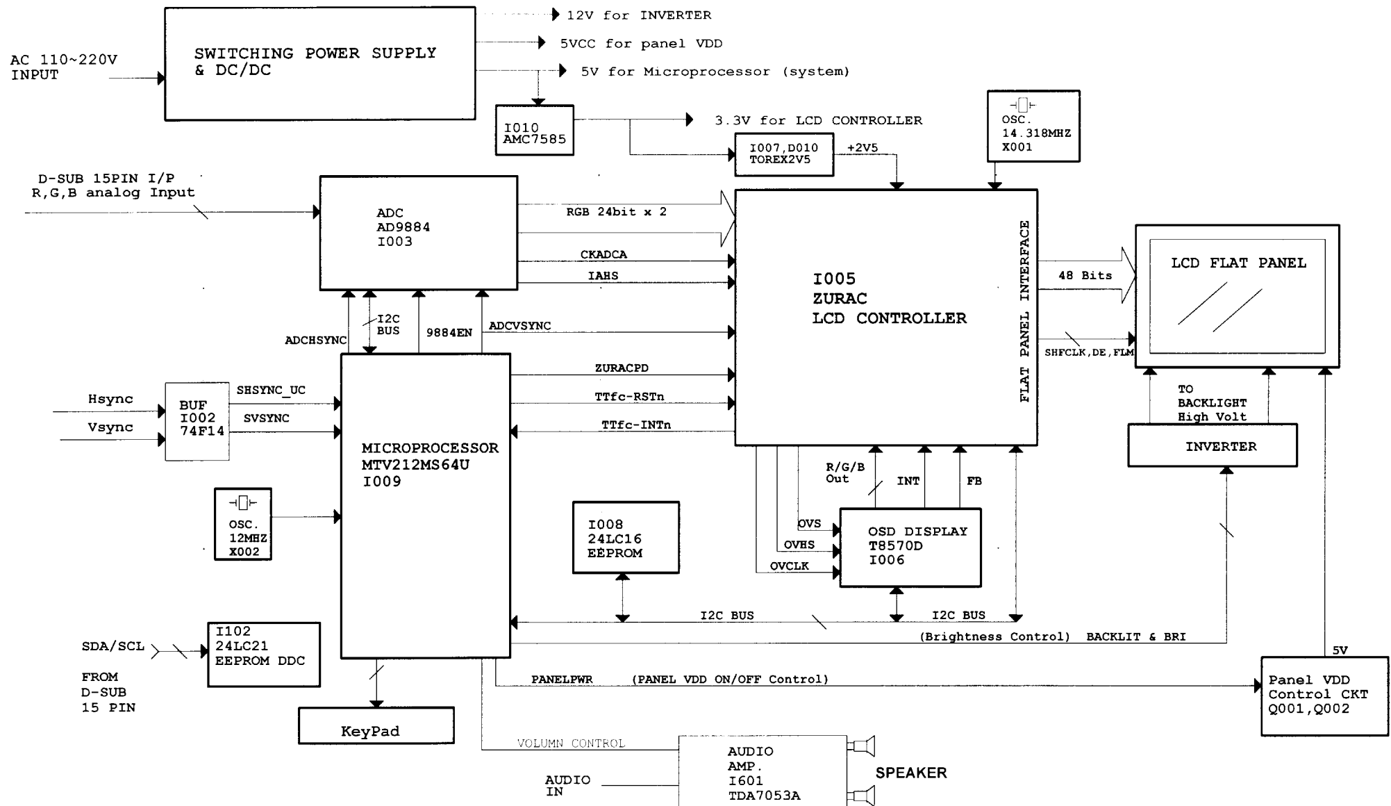
15 inch LCD MONITOR FLOW CHAR
