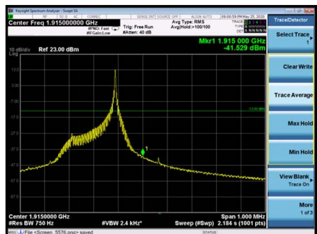
NB-IOT Band 25 QPSK 3.75kHz 1@47 CH-High
