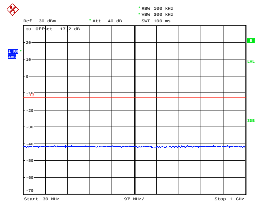
NB-IOT Band 2 CH-High 30MHz~1GHz
