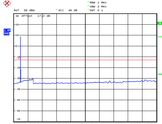
NB-IOT Band 2 CH-High 1GHz ~20GHz
