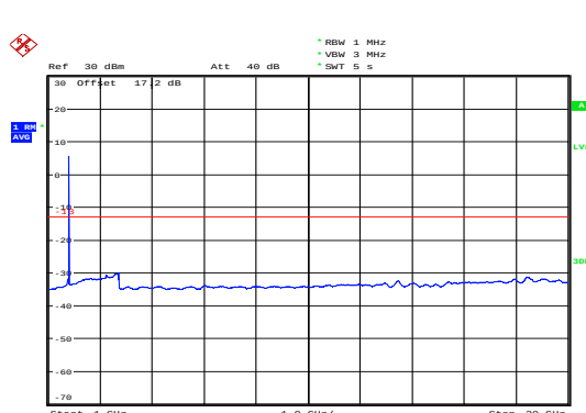
LTE Band 4 1.4MHz CH- Middle 1GHz ~20GHz
