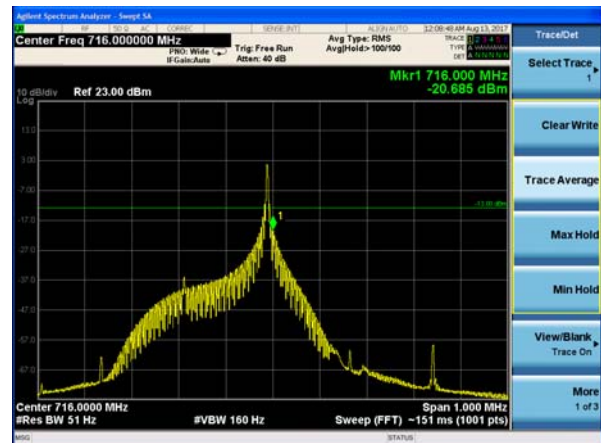
NB-IOT Band 12 BPSK 15kHz 1@11 CH-High
