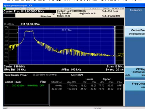
LTE Band 26 16QAM 100%RB CH26740 10M
