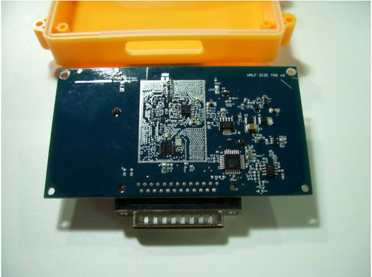
Figure 2: RF Board (Bottom View)
