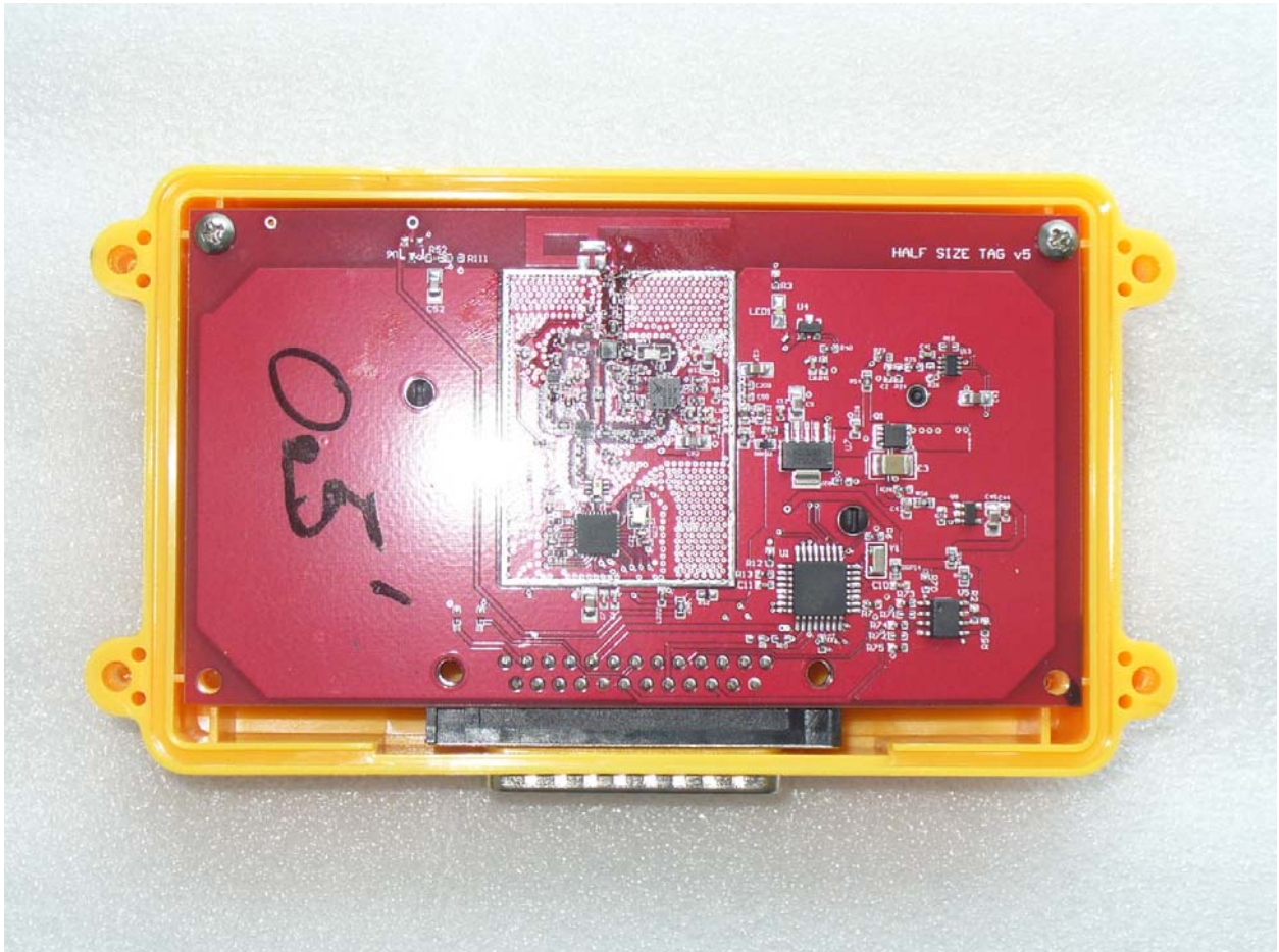
Figure 3: Internal View
