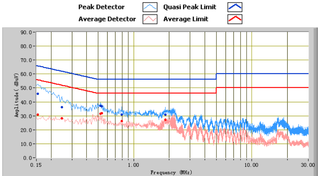
Phase Neutral Plot at AC 240V 50Hz
