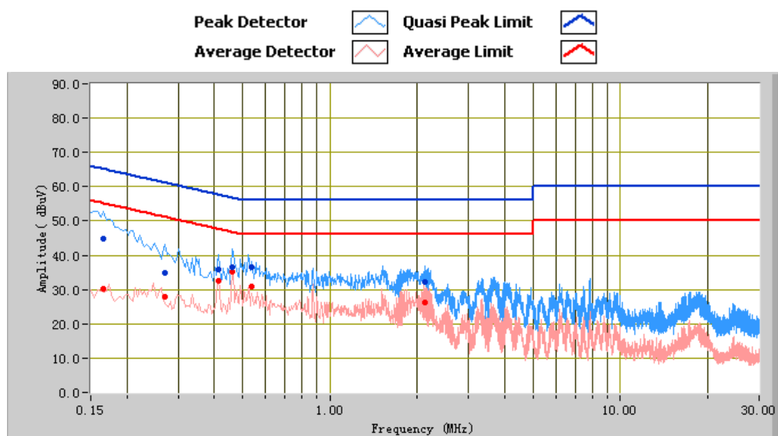
Phase Neutral Plot at AC 240V 50Hz
