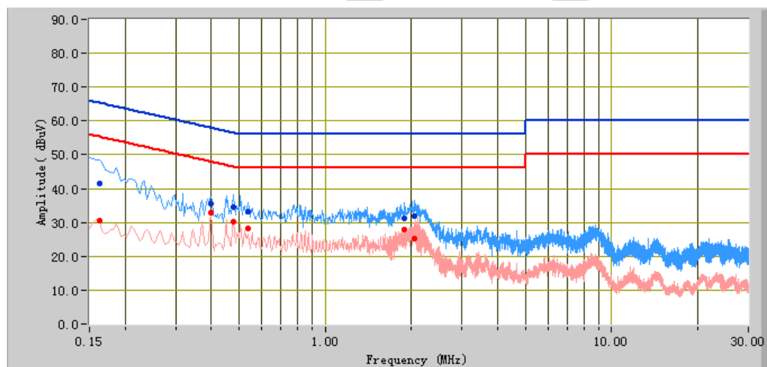
Phase Neutral Plot at AC 120V 60Hz
