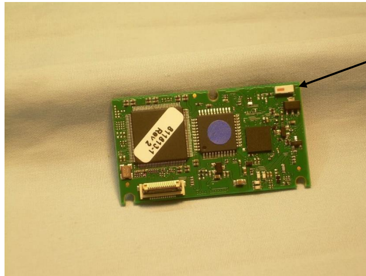
Photograph 3 – Bottom View of the PCB
