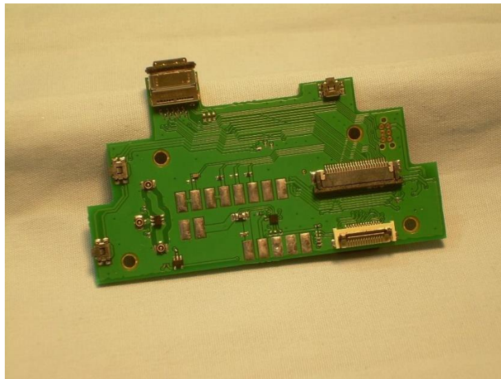
Photograph 6 – Back View of Keypad PCB
