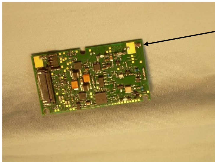
Photograph 2 – View of the Circuitry under the RF Shield
