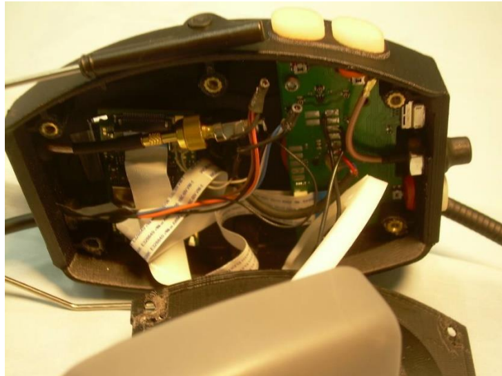
Photograph 4 – View of the PCB inside of Housing
