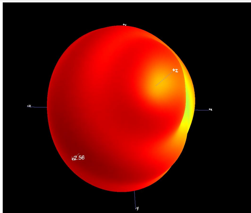
B1.2 3D Pattern for 916MHz
