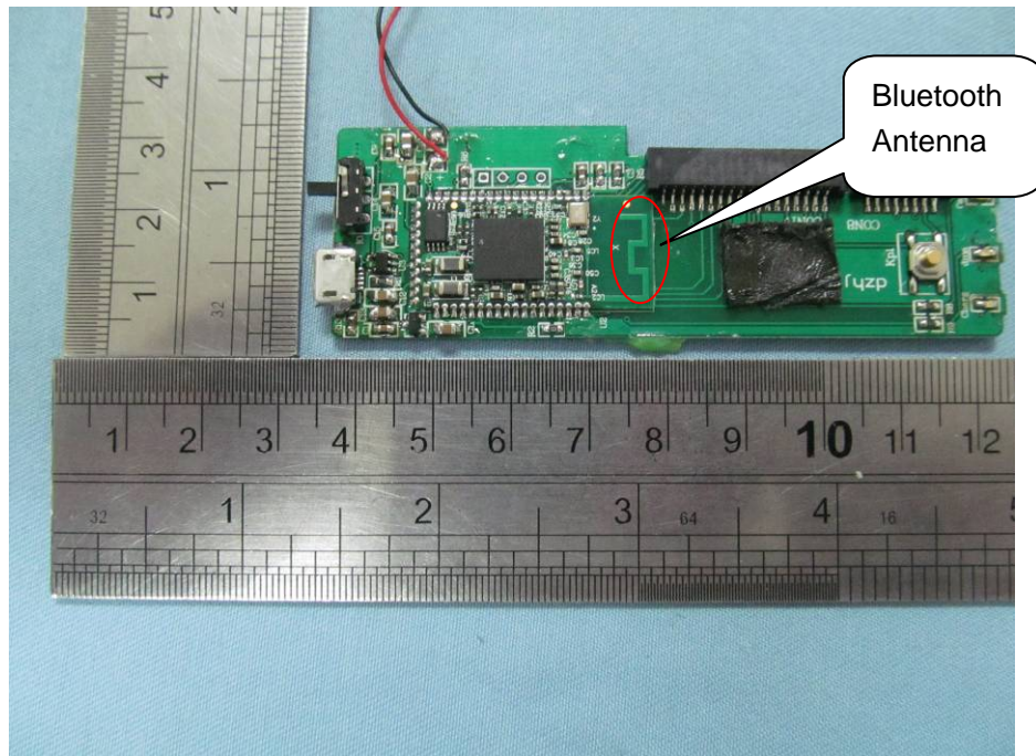
FRONT VIEW-2 OF PCB
