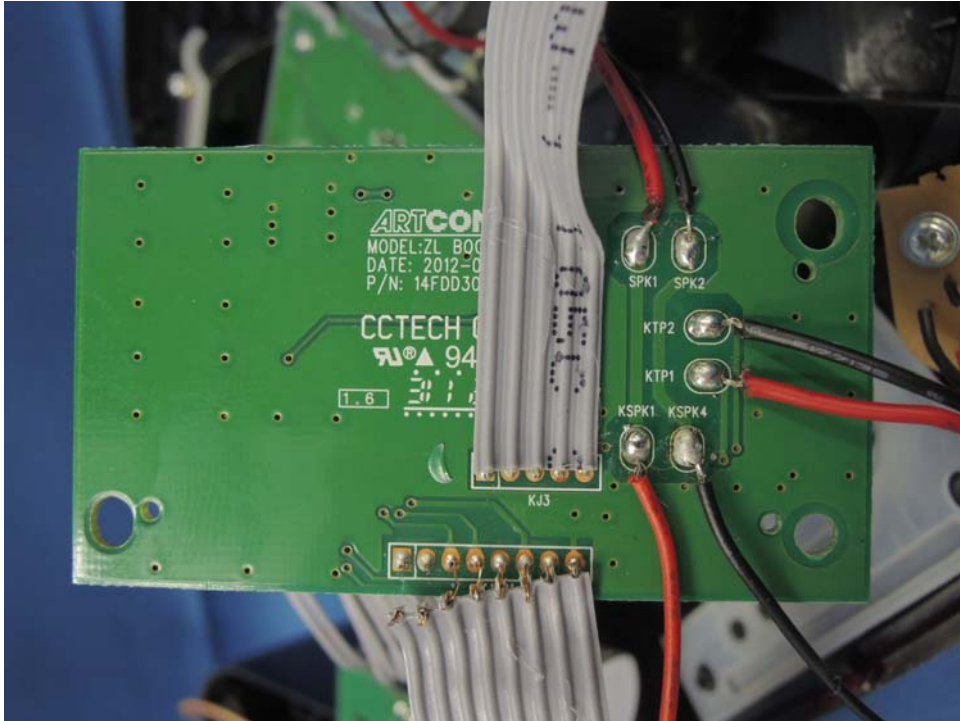
Base Unit Page Key rear side (View 2)
