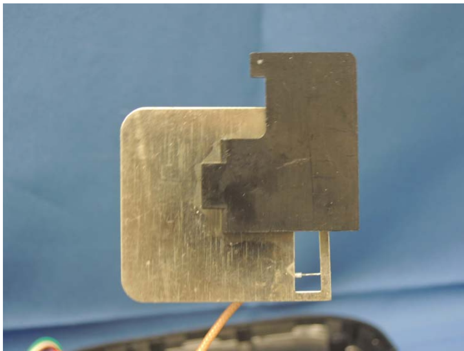
Base Unit Antenna 2 (View 1)
