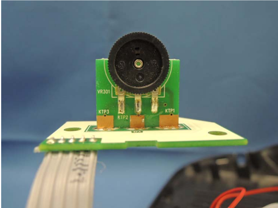
Base Unit Volume board front side (View 2)
