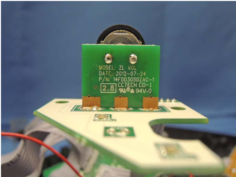
Base Unit Volume board front side (View 3)
