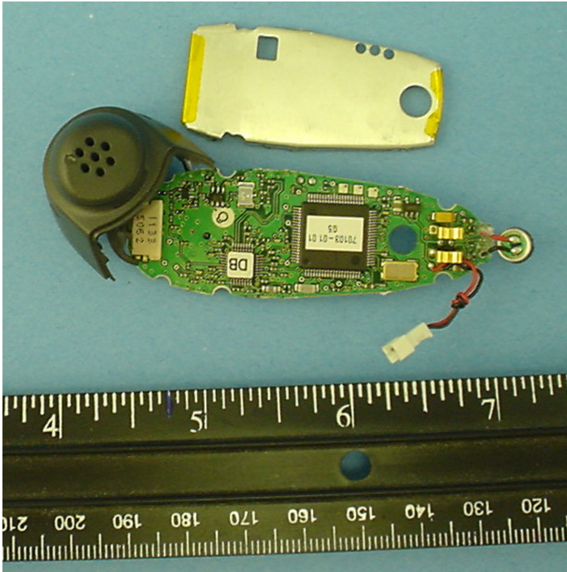
CS55YYYY side A, with detached shield.
