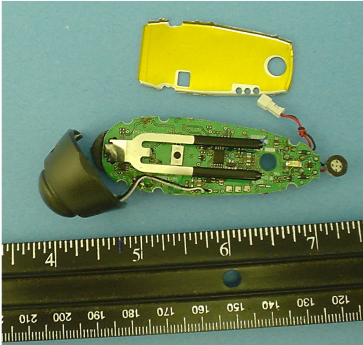
AL8CS55YYYY B side, with detached shield
