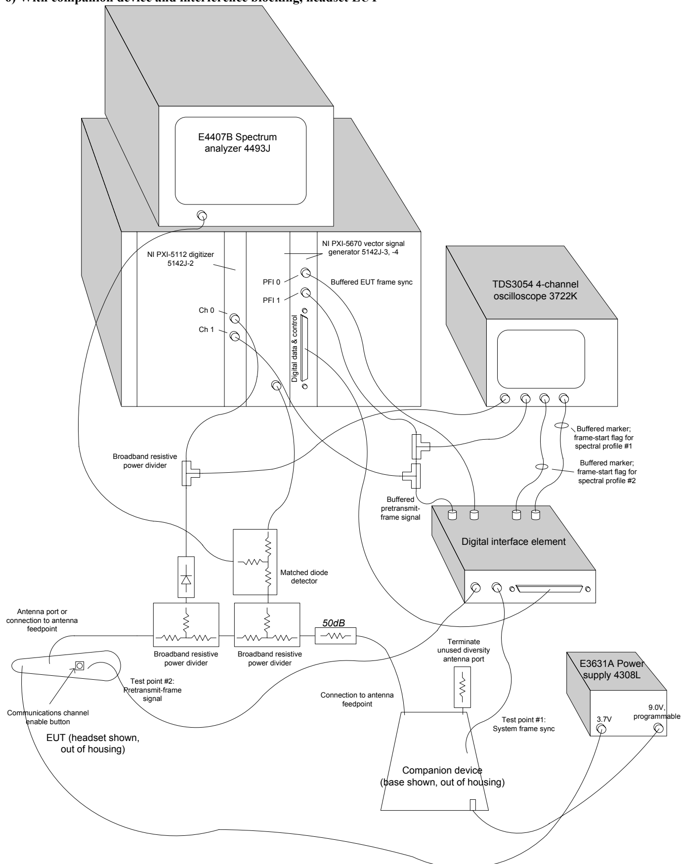
Fig. 2 - Detail of connections to headset EUT for the tests of clause 7 and clause 8 of V3.3 (draft) C63.17-2005, for configuration 6, With companion device and interference blocking, headset EUT . All RF cables are RG142LL.
