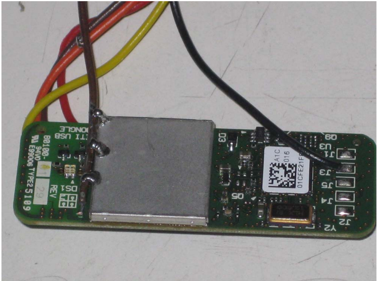
Fig. 6 – Detail of the attachment of the RF connection for conducted measurements.
