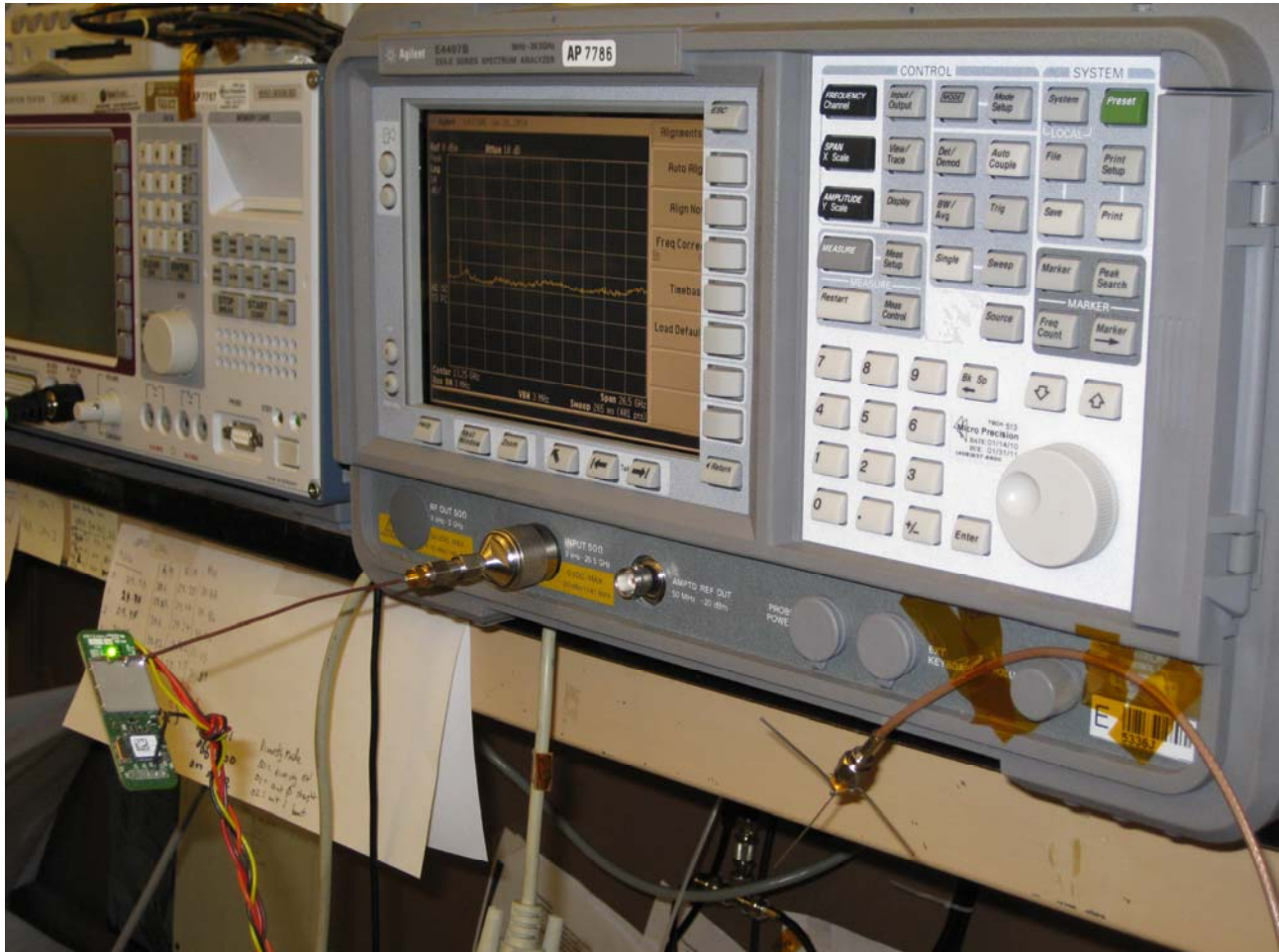
Fig. 5 - Base EUT in direct connection with spectrum analyzer and radiated connection with base companion device, for the tests of clause 6.1.
