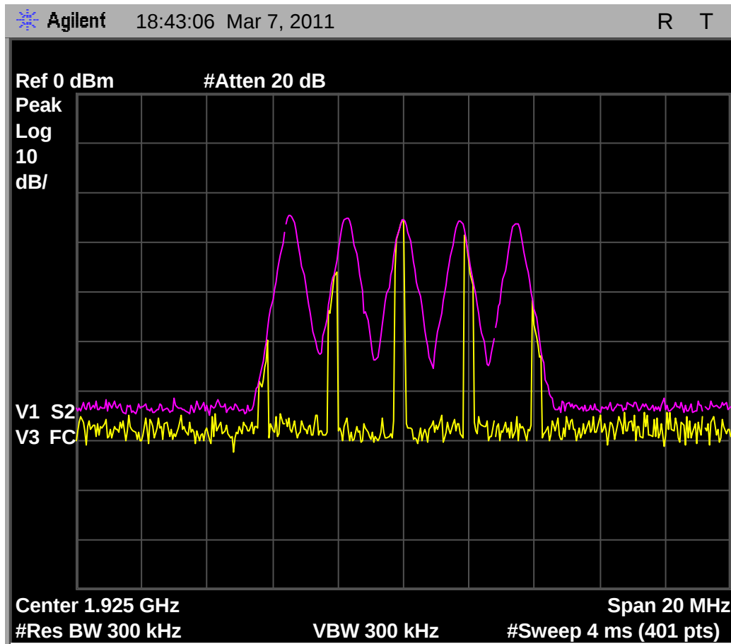
Fig. 56 - Transmit spectrum of 35uS interference pulses in each timeslot for each carrier, with Base EUT deferring due to interference pulses of T_U + U_M + 6\text{dB} .
