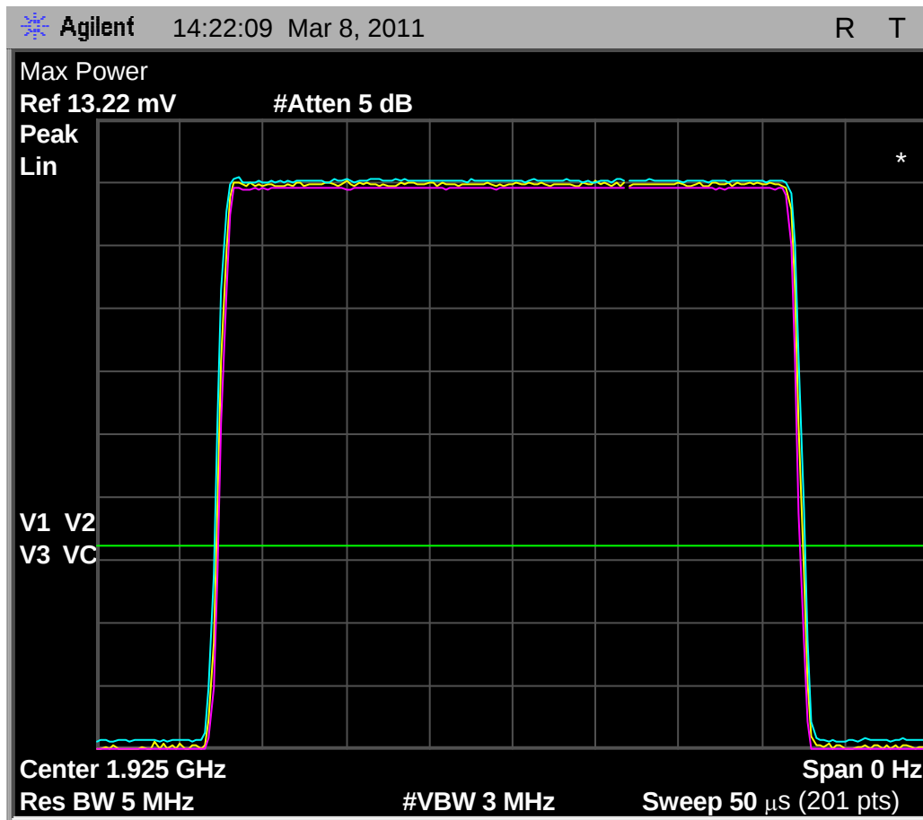
Fig. 55 - 35uS interference pulse for 7.5(d), duration and amplitude variation over the duration of the pulse and over multiple pulses. Spectrum analyzer is set to linear response.
