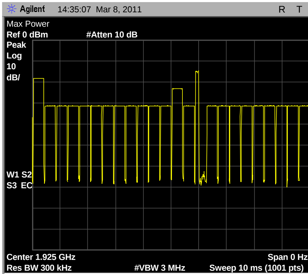
Fig. 58 – Zero-span (single frequency receiver mode) sweep of TDMA interference on carrier at 1924.993MHz, f_1 , with Base EUT beacon transmissions in the single unblocked timeslot.
