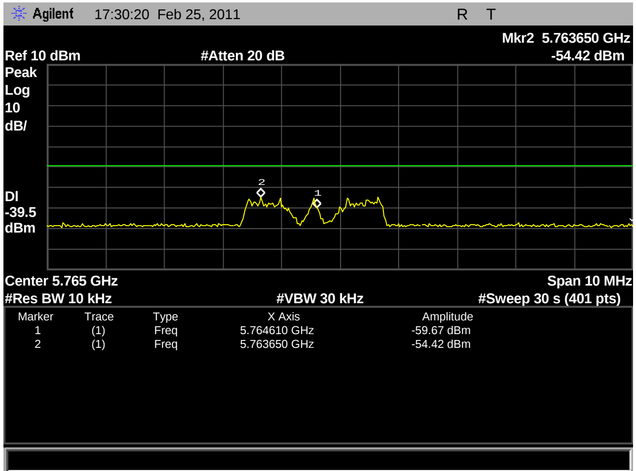
Fig. 28 – Base EUT out-of-band emissions in the region around the 3rd harmonic, with the Base EUT transmitting on the lowest carrier, 1921.536MHz.
