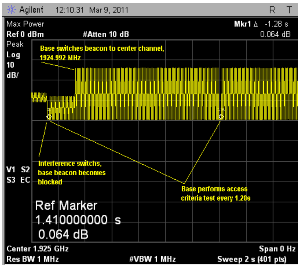
Fig. 62 – Zero span spectrum analyzer display of Base EUT pausing the transmission of signaling to check access criteria, finding the channel no longer meets the access criteria, and resuming transmissions on an alternate carrier.
