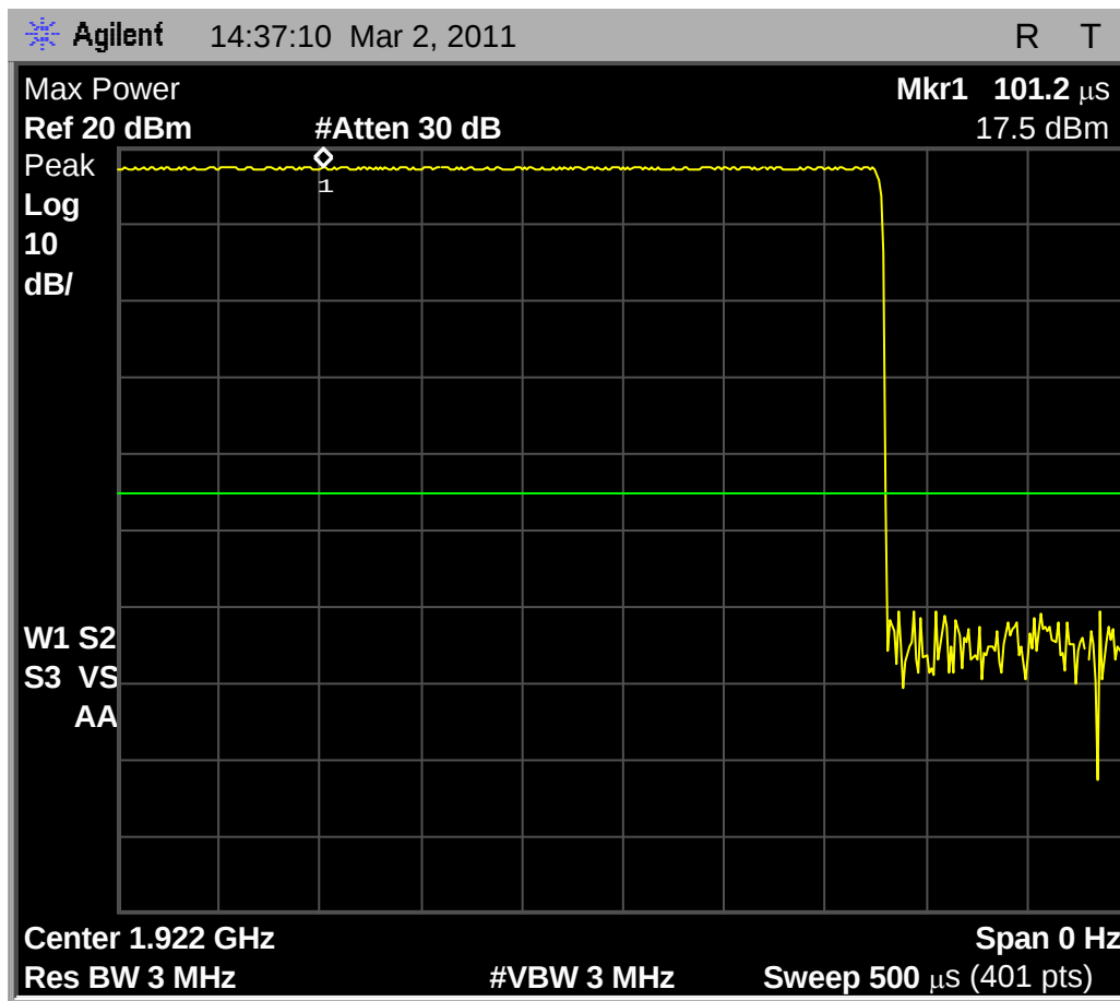
Fig. 7 - Base EUT transmit power received by spectrum analyzer configured according to the requirements of clause 6.1.2 of C63.17-2006, low carrier. Maximum observed transmit power is 17.5 dBm.
