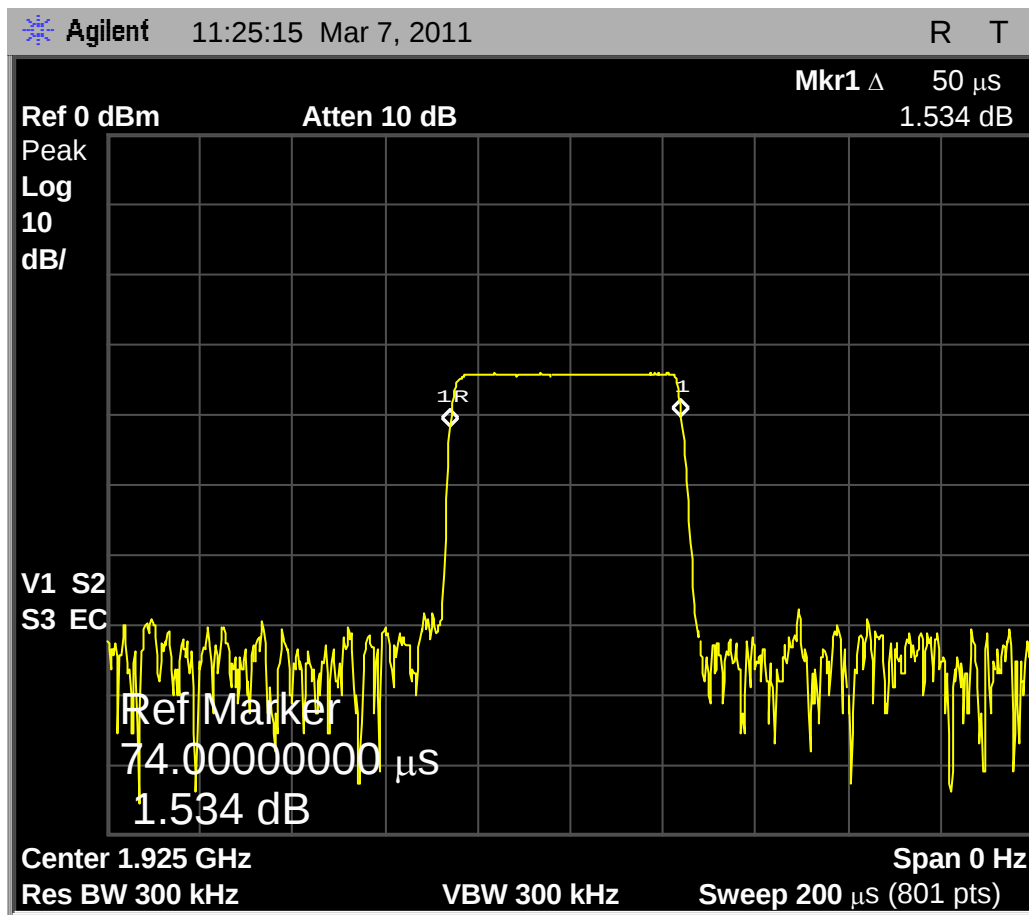
Fig. 49 - Interference pulse, one frame shown, for the test of 7.5(c).
