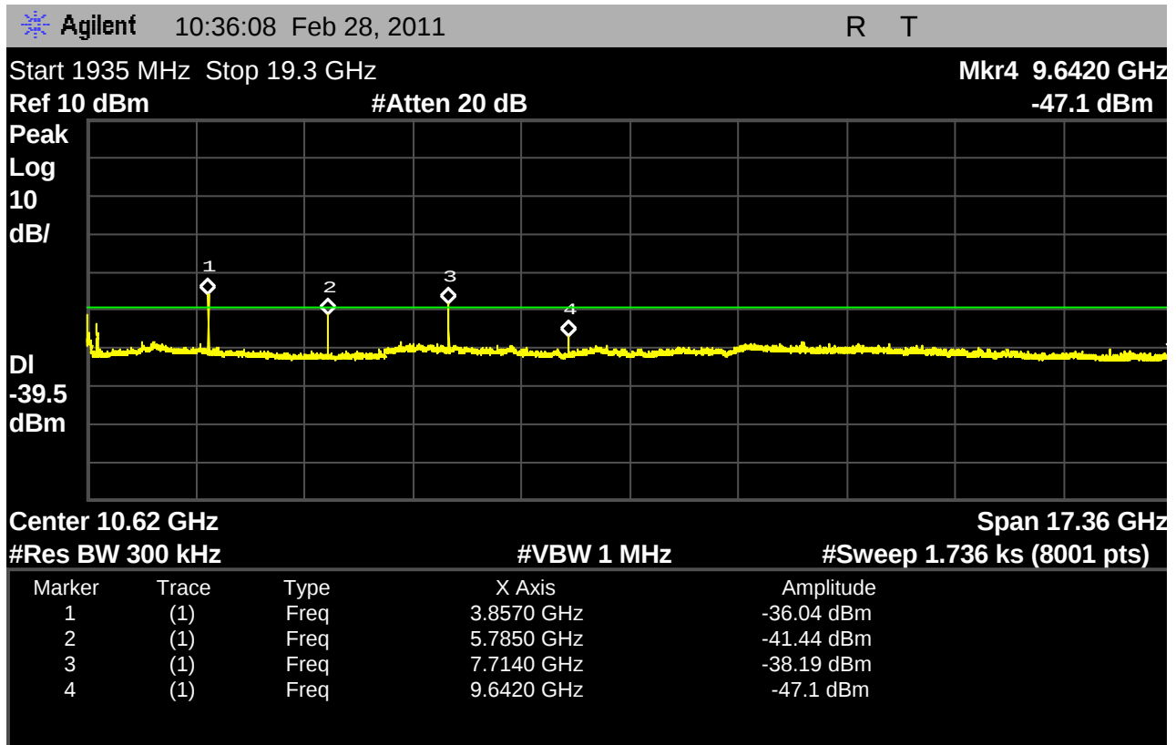
Fig. 34 – Base EUT out-of-band emissions including the regions from 1935MHz to 19.3GHz with the Base EUT transmitting on the highest carrier, 1928.448MHz.
