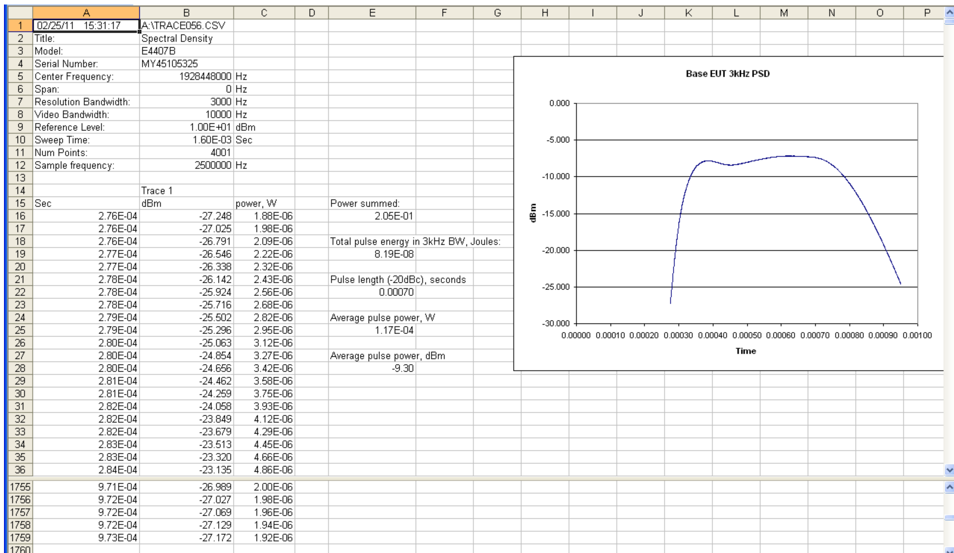
Fig. 18 – Screenshot of Excel file showing PSDlimit calculations for Base EUT, high carrier; -9.3dBm.
