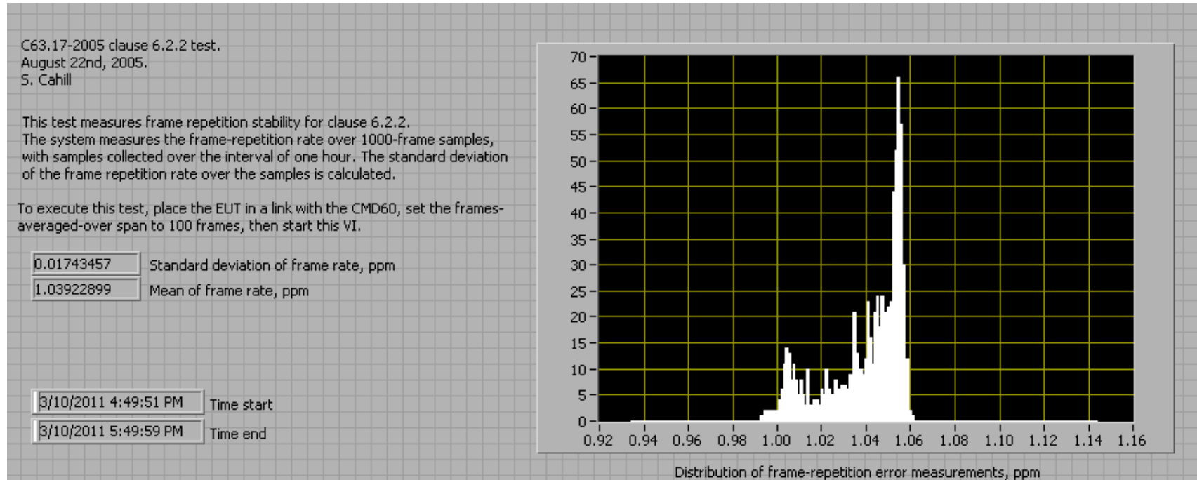
Fig. 41 - Test of Base EUT according to the conditions of clause 6.2.2 for frame repetition rate stability
