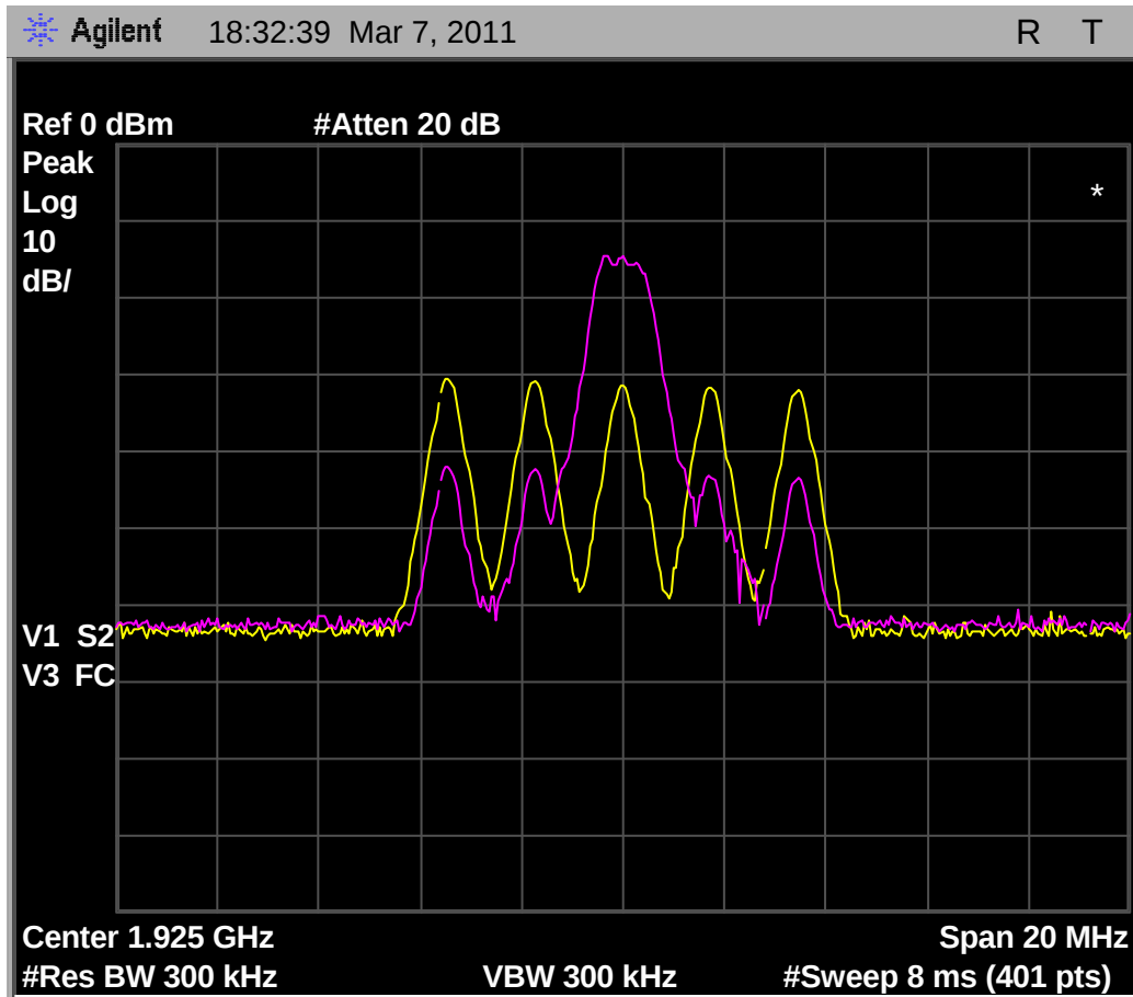
Fig. 53 - Transmit spectrum of 50uS interference pulses, with Base EUT no longer deferring with interference pulses of level T_U - U_M .
