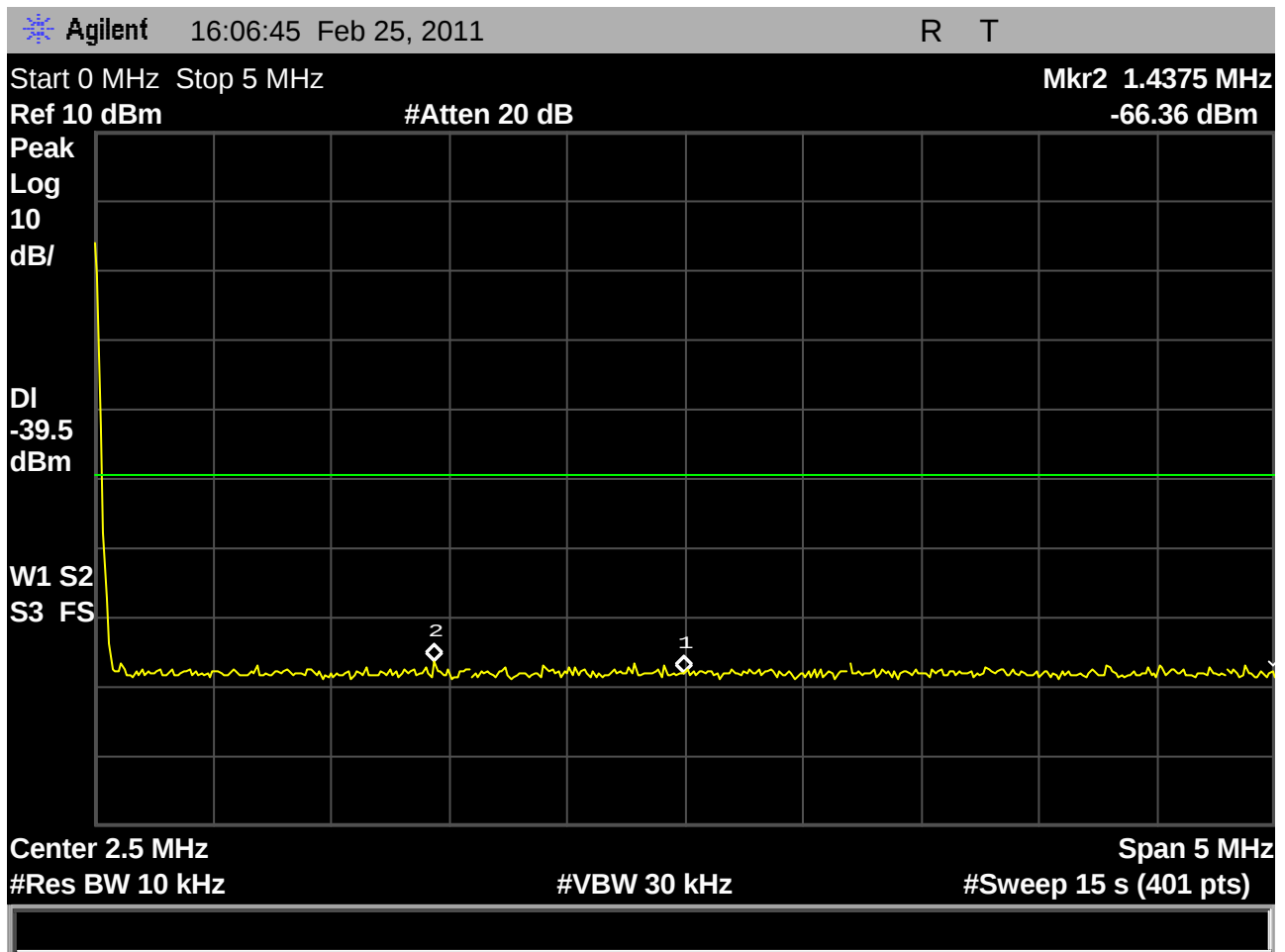
Fig. 22 – Base EUT out-of-band emissions showing the regions from DC to 5MHz, with the transmitter using the lowest carrier, 1921.536MHz.
