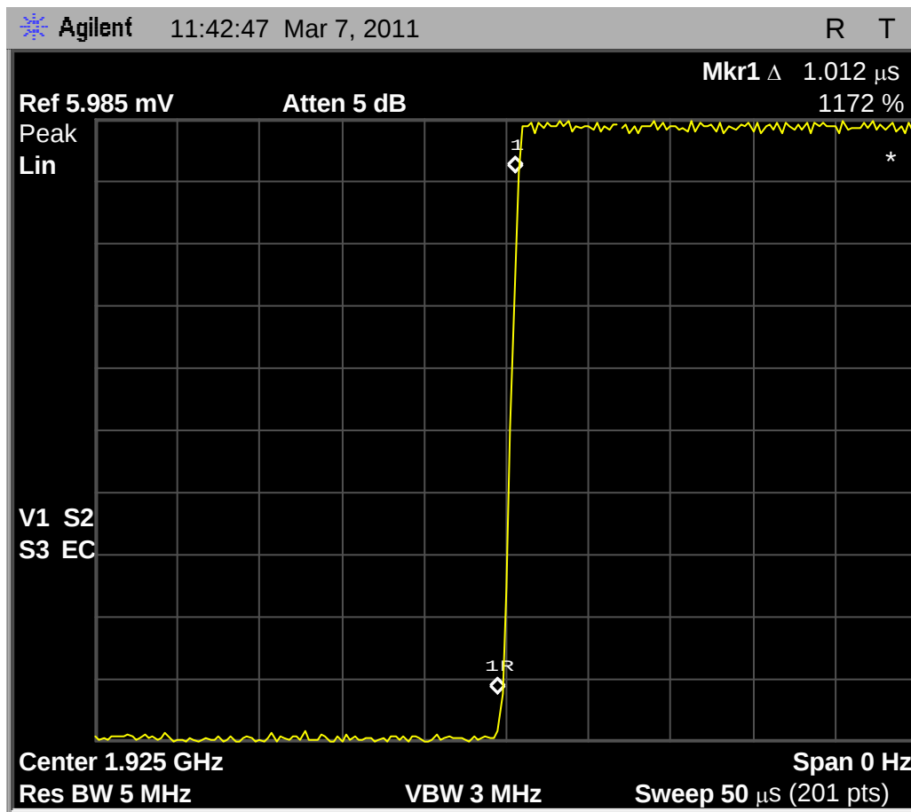
Fig. 50 - Rise time of interference pulse, per the requirements of 7.5 for less than 1uS for 10% to 90% transition.
