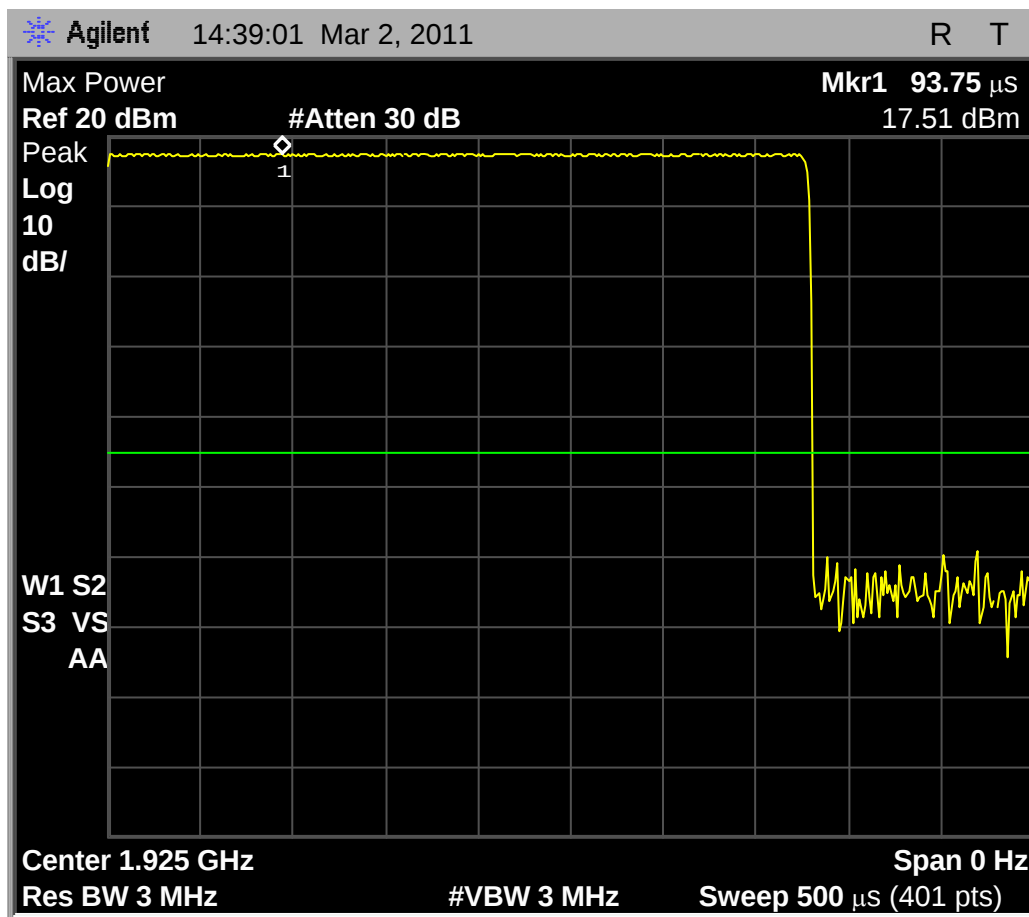
Fig. 8 - Base EUT transmit power received by spectrum analyzer configured according to the requirements of clause 6.1.2 of C63.17-2006, mid carrier. Maximum observed transmit power is 17.51 dBm
