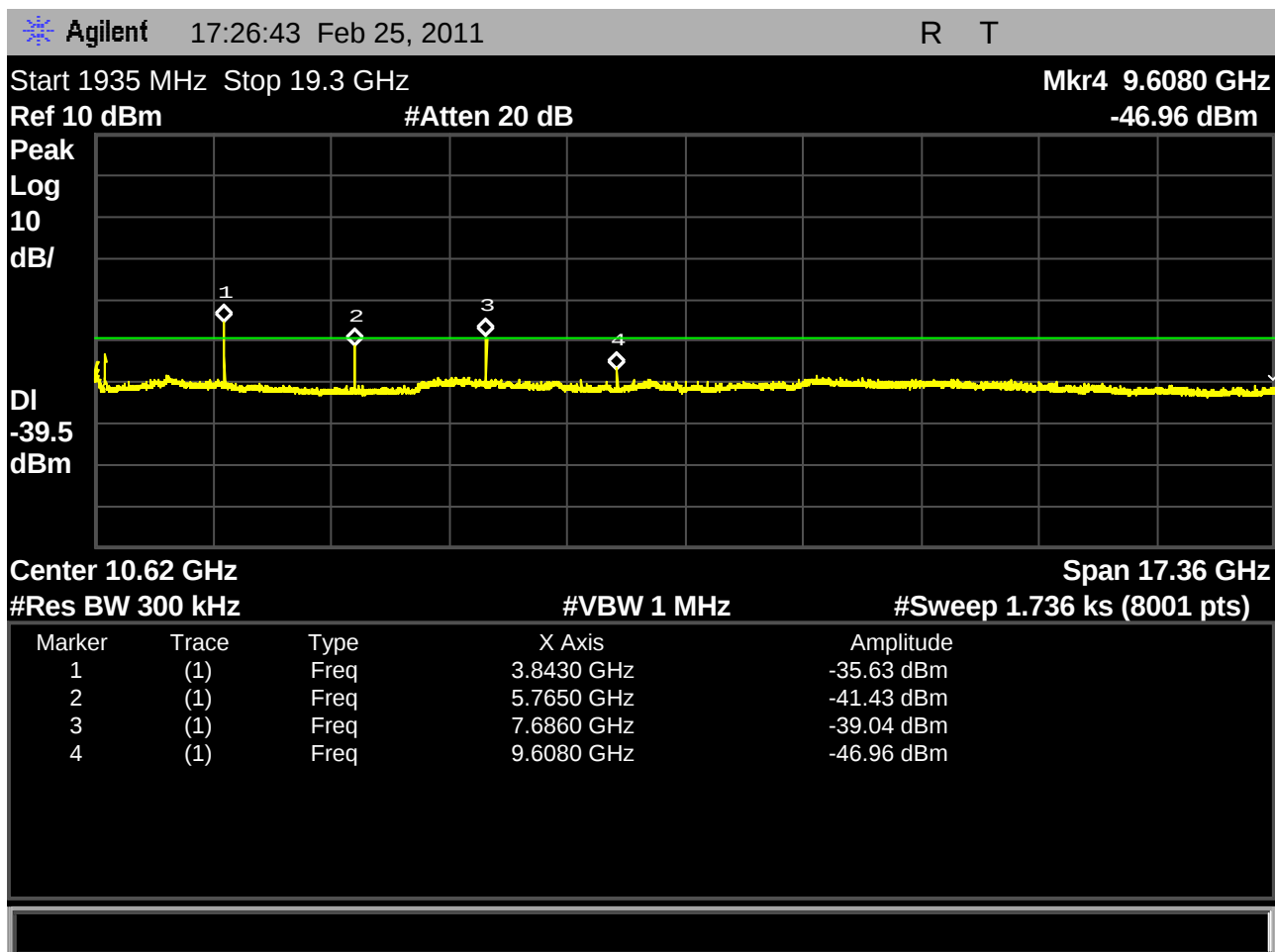
Fig. 26 – Base EUT out-of-band emissions including the regions from 1935MHz to 19.3GHz with the Base EUT transmitting on the lowest carrier, 1921.536MHz.
