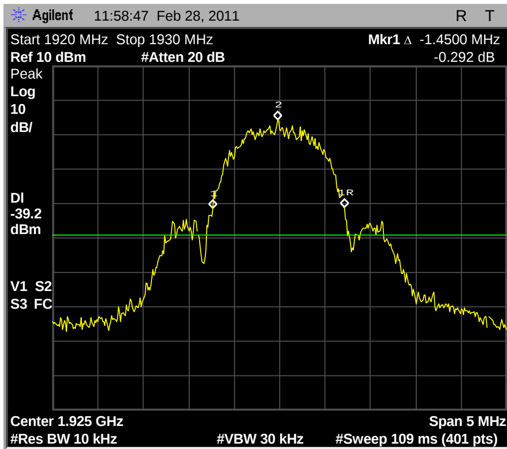
Fig. 68 - Base EUT in low power WBM, 1.45MHz emissions bandwidth on mid carrier vs. 1.42MHz in max power normal mode.
