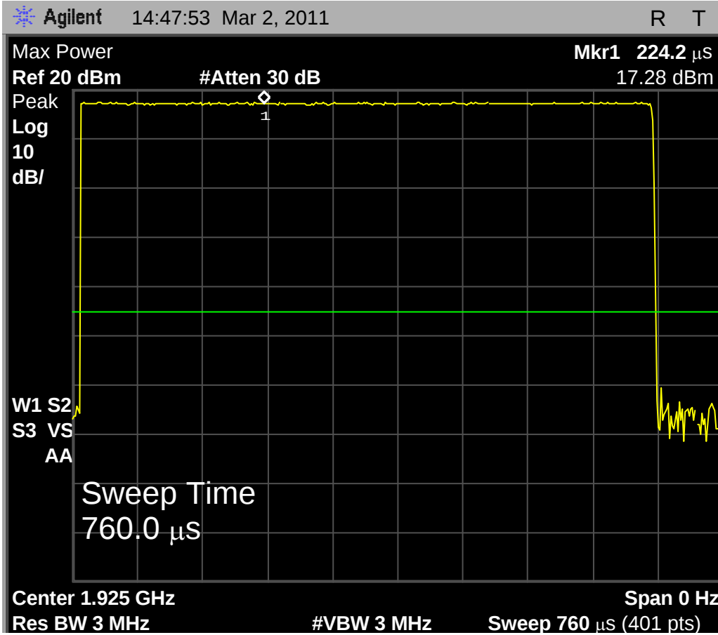
Fig. 65 - Base EUT transmit power received by spectrum analyzer configured according to the requirements of clause 6.1.2 of C63.17-2006, mid carrier. Maximum observed transmit power is 17.28 dBm in WBM; output power for normal mode on mid channel was 17.51dBm ( P_{max} = 20.8 dBm).
