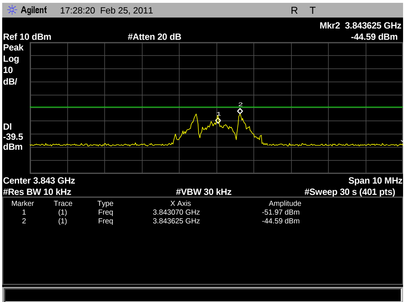
Fig. 27 – Base EUT out-of-band emissions in the region around the 2 nd harmonic, with the Base EUT transmitting on the lowest carrier, 1921.536MHz.
