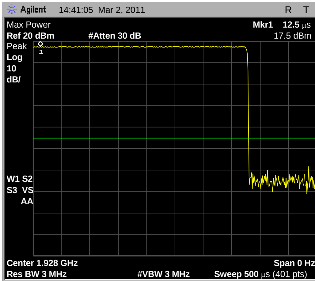
Fig. 9 - Base EUT transmit power received by spectrum analyzer configured according to the requirements of clause 6.1.2 of C63.17-2006, high carrier. Maximum observed transmit power is 17.5 dBm.
