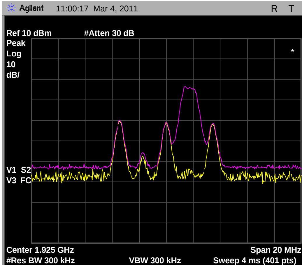
Fig. 47 - Emissions and interference profile spectrum, Base EUT, test 7.3.3(e).
