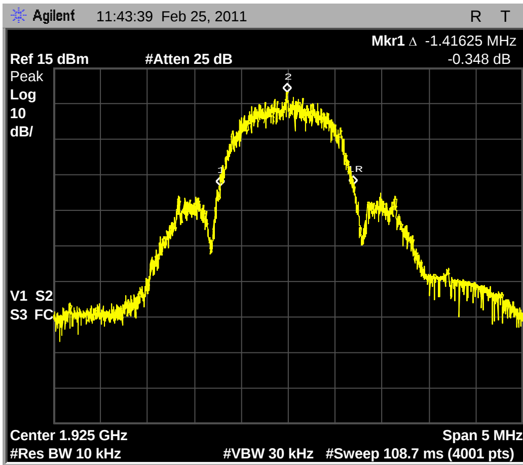
Fig. 11 - Base EUT, 1.45MHz emissions bandwidth on middle carrier, 1.41625 MHz.
