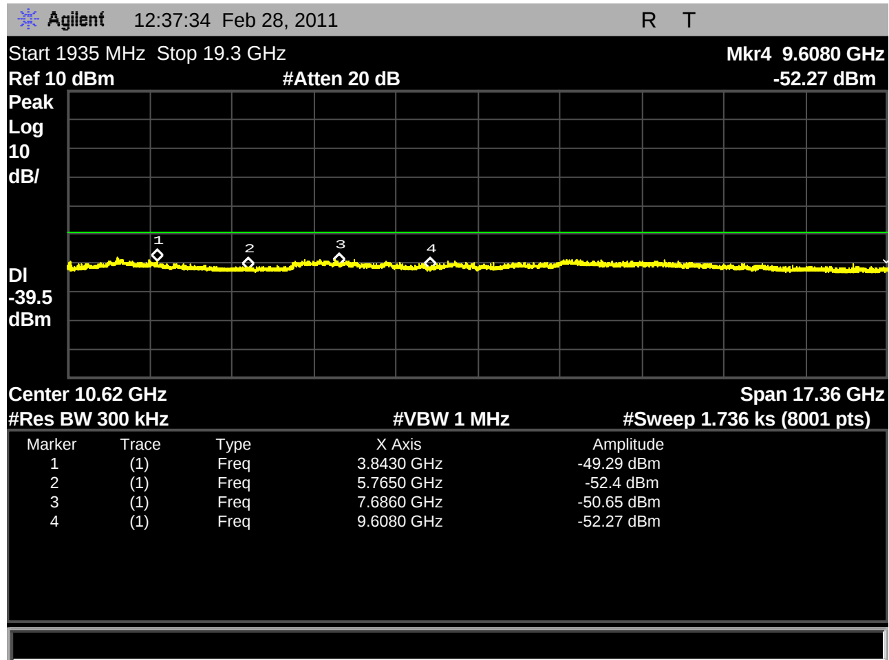
Fig. 70 - - Base EUT in minimum power WBM on low carrier. All harmonics are below specification in minimum power, even when measured in the 300kHz (greater) resolution bandwidth.
