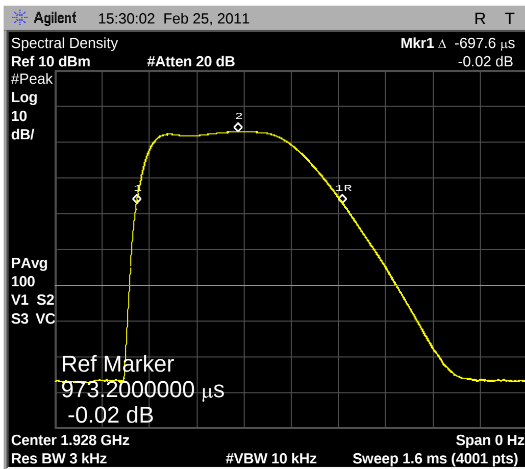
Fig. 17 – Zero-span sweep for Base EUT, high carrier, for 3kHz maximum power spectral density. The peak level is at -7.154dBm, and the interval between samples at the -20dB points is 697.6us.
