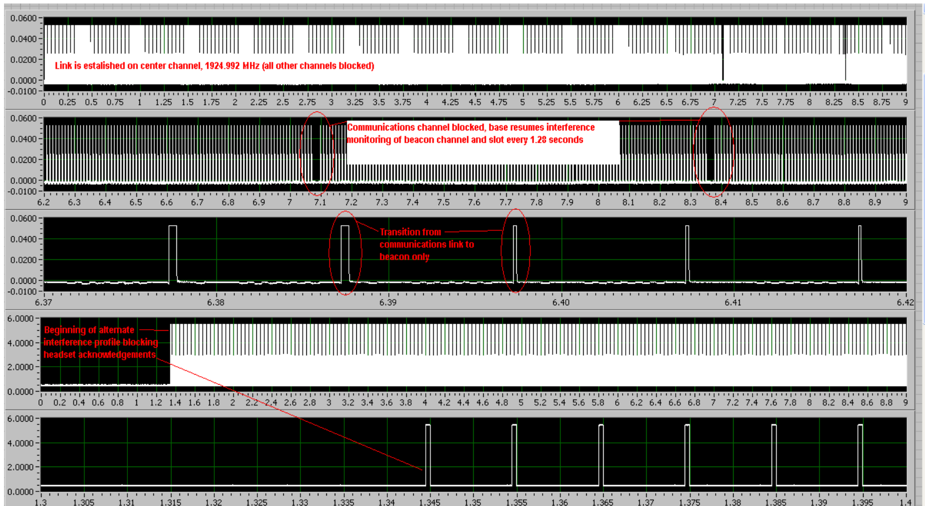
Fig. 64 – Capture of Base EUT transmission changing from communications link to beacon only.
