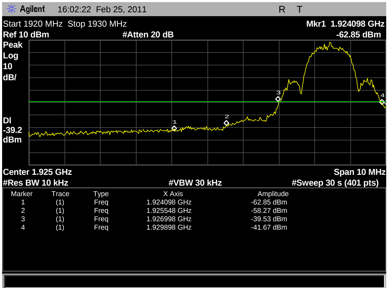
Fig. 21 - Spectrum analyzer screenshot for transmit emissions showing in-band unwanted emissions with the Base EUT transmitter at the highest carrier, 1928.448MHz, according to the requirements of 6.1.6.1.
