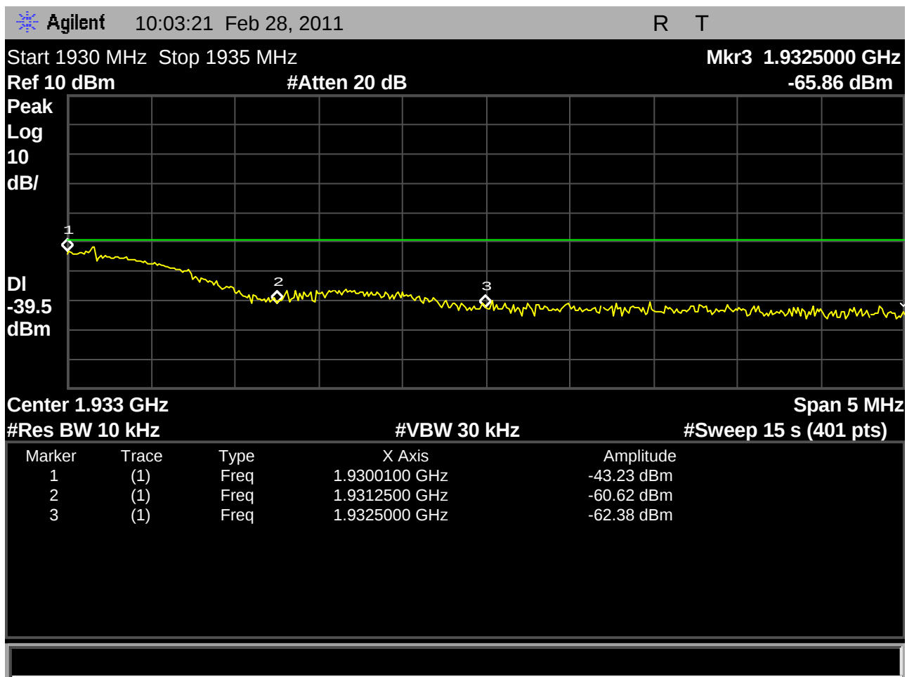
Fig. 33 – Base EUT out-of-band emissions showing the regions from band edge to +1.25MHz, and from +1.25MHz to +2.5MHz, with the Base EUT transmitting on the highest carrier, 1928.448MHz. Note the green display line is the spec limit marker only for the region outside +2.5MHz.
