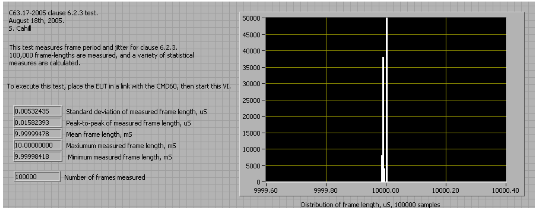
Fig. 42 - Test of Base EUT for frame period and jitter, according to the requirements of clause 6.2.3.
