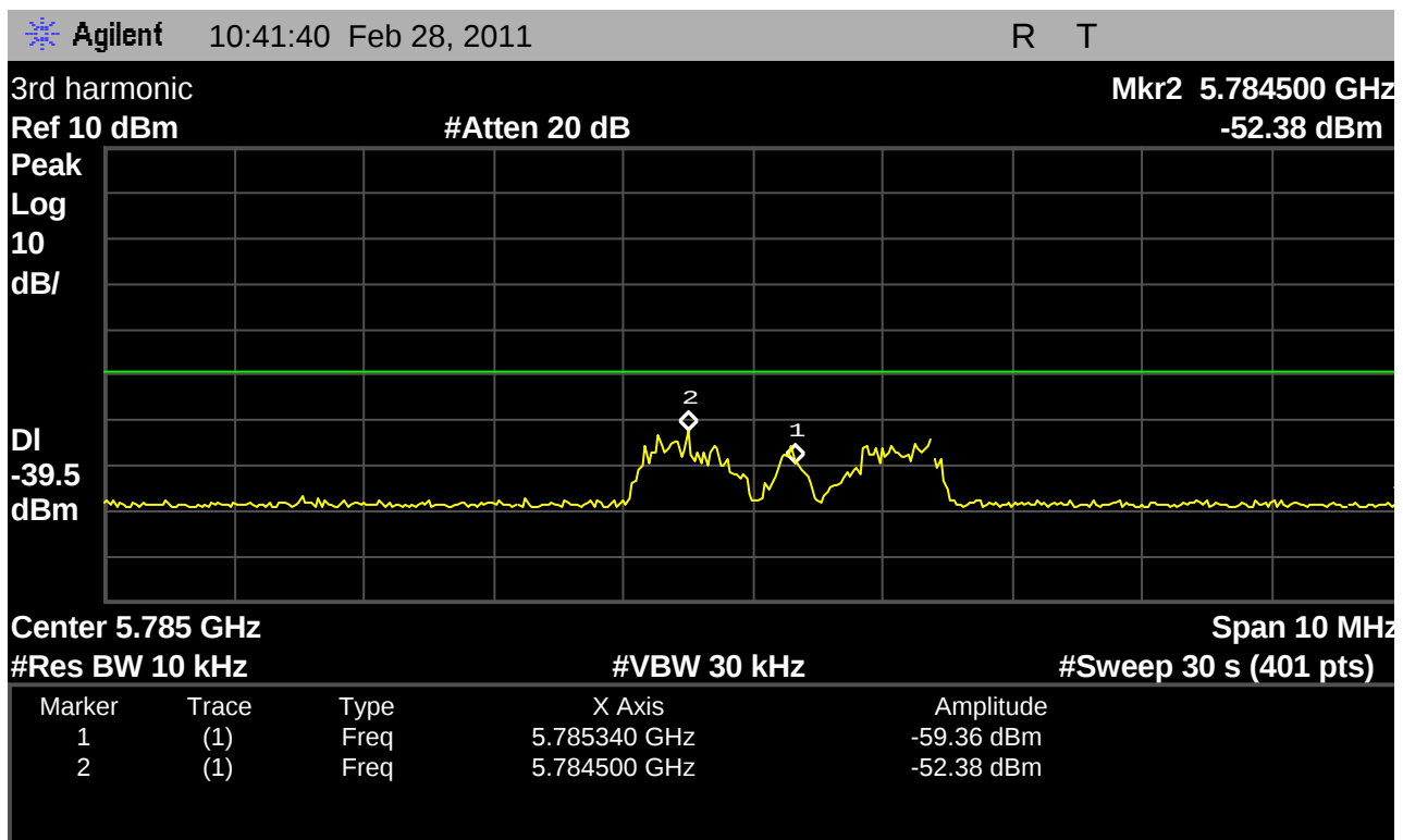
Fig. 36 – Base emissions measured in 10kHz resolution bandwidth in the region where the 1935MHz to 19.3GHz sweep at 300kHz observed a 3 rd harmonic response, for the Base transmitting on the high carrier, 1928.448MHz. A peak of -52.38dBm is measured in the specified resolution bandwidth, a margin of 12.88dB from the -39.5dBm spec limit.
