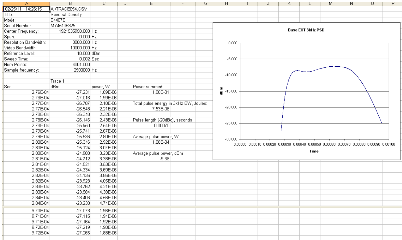
Fig. 14 – Screenshot of Excel file showing PSDlimit calculations for Base EUT, low carrier; -9.66dBm
