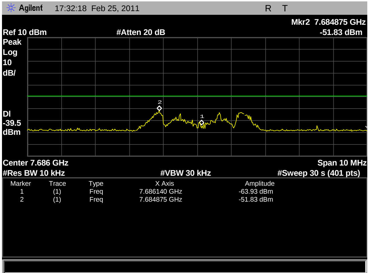
Fig. 29 – Base EUT out-of-band emissions in the region around the 4th harmonic, with the Base EUT transmitting on the lowest carrier, 1921.536MHz.
