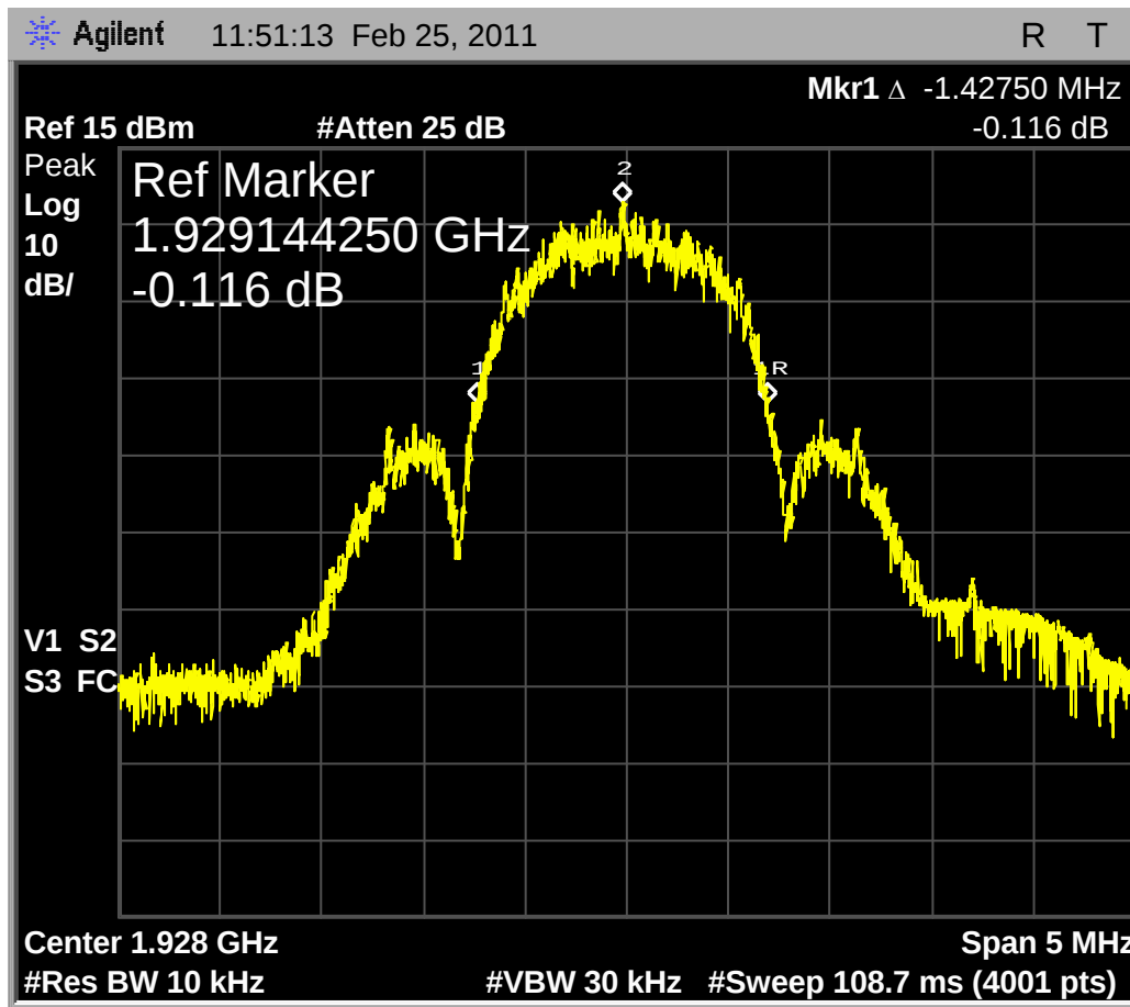
Fig. 12 - Base EUT, 1.44MHz emissions bandwidth on high carrier, 1.4275 MHz.
