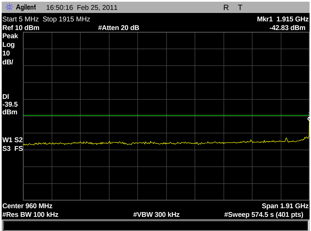
Fig. 23 – Base EUT out-of-band emissions showing the region from 5MHz to 1915MHz, with the transmitter using the lowest carrier, 1921.536MHz.
