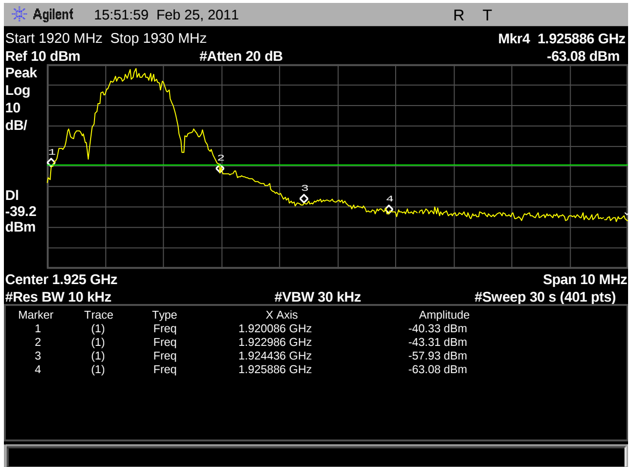
Fig. 19 - Spectrum analyzer screenshot for transmit emissions showing in-band unwanted emissions with the Base EUT transmitter at the lowest carrier, 1921.536MHz, according to the requirements of 6.1.6.1.
