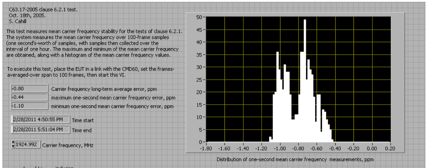
Fig. 38 - Measured one-second mean carrier frequency, Base EUT, and observed maximum, average value and observed minimum of the mean carrier frequency.
