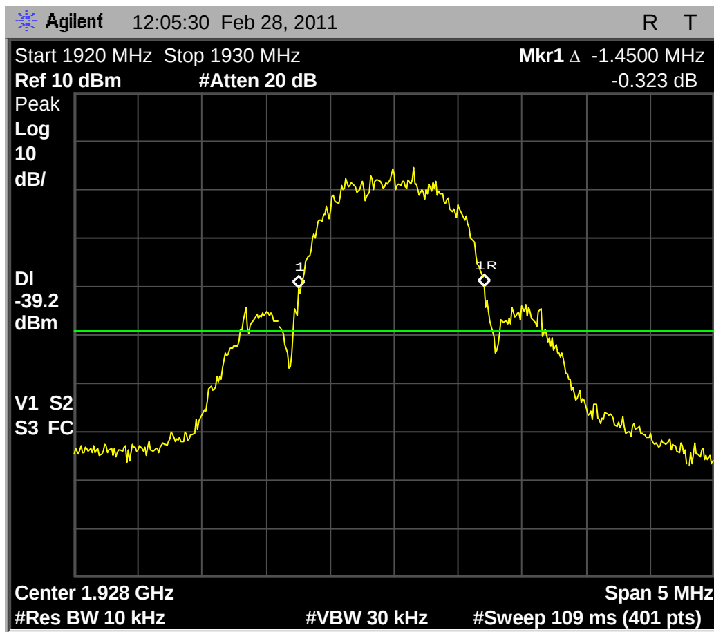
Fig. 69 - Base EUT in low power WBM, 1.45MHz emissions bandwidth on high carrier vs. 1.43MHz in max power normal mode.
