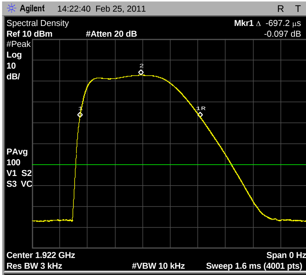
Fig. 13 – Zero-span sweep for Base EUT, low carrier, for 3kHz maximum power spectral density. The peak level is at -7.246dBm, and the interval between samples at the -20dB points is from 697.2us.
