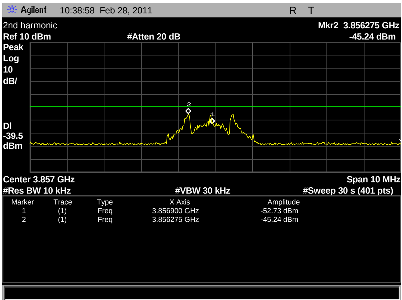
Fig. 35 – Base emissions measured in 10kHz resolution bandwidth in the region where the 1935MHz to 19.3GHz sweep at 300kHz observed a 2 nd harmonic response, for the Base transmitting on the high carrier, 1928.448MHz. A peak of -45.24dBm is measured in the specified resolution bandwidth, a margin of 5.74dB from the -39.5dBm spec limit.
