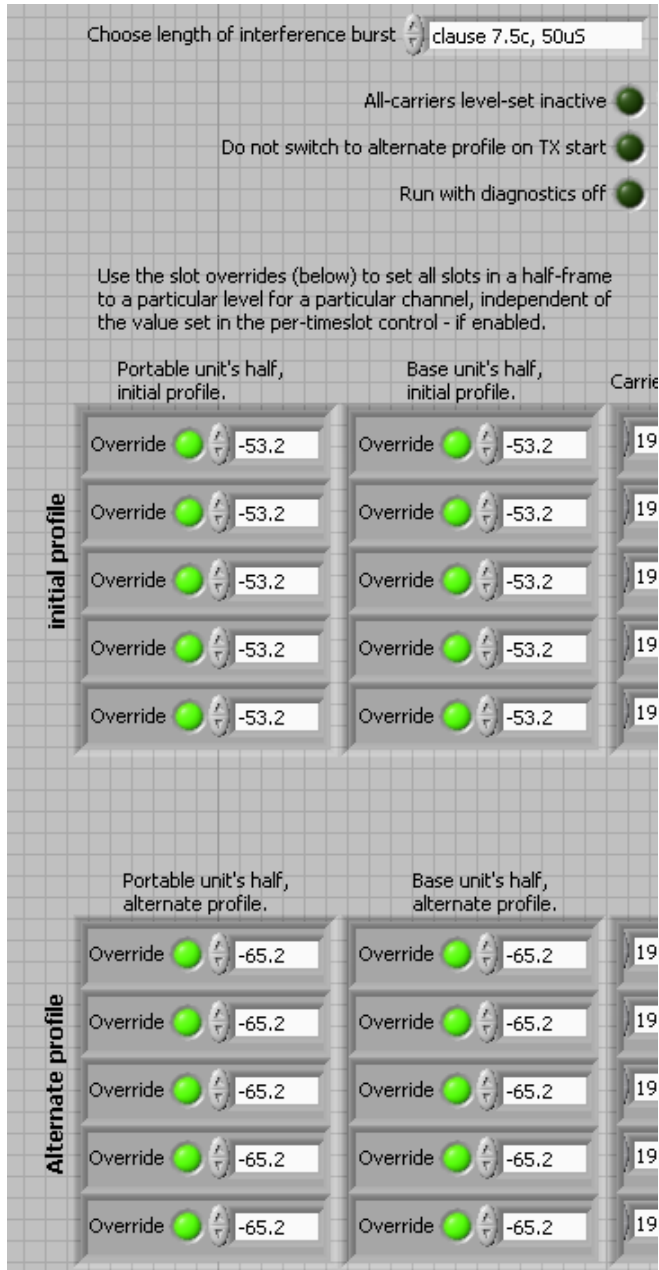
Fig. 48 - Control panel for multi-carrier interference generator, set to 50uS pulses in all timeslots on all carriers, for the test of 7.5(c).
