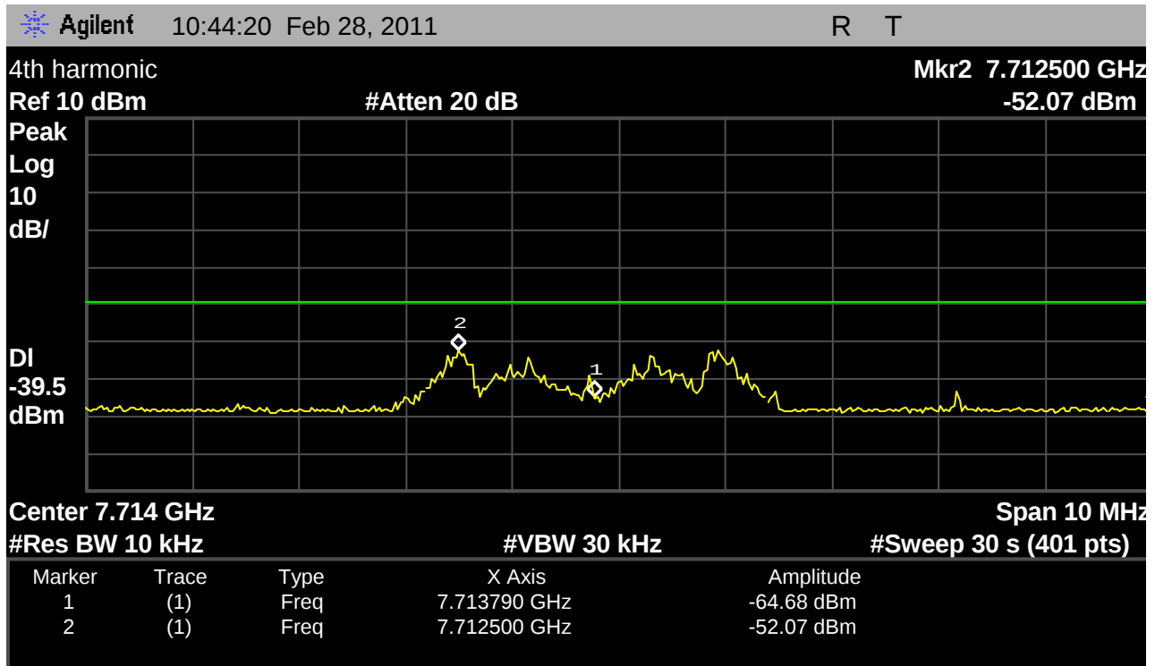
Fig. 37 – Base EUT out-of-band emissions in the region around the 4 th harmonic, with the Base EUT transmitting on the highest carrier, 1928.448MHz.
