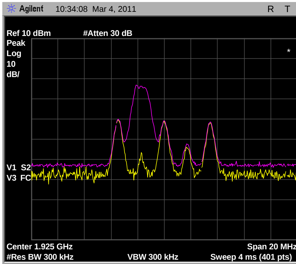
Fig. 44 - Emissions and interference profile spectrum, Base EUT, test 7.3.3(b).
