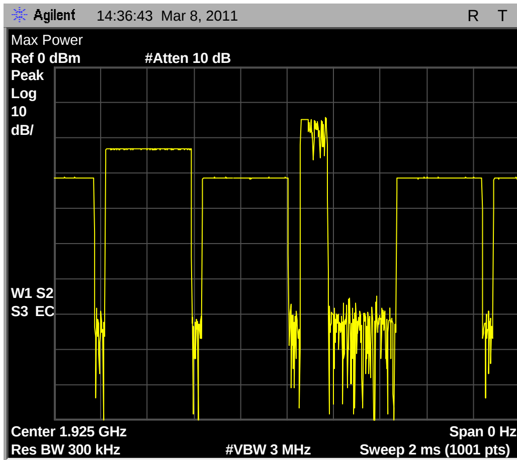
Fig. 59 – Zero-span (single frequency receiver mode) sweep of TDMA interference on carrier at 1924.993MHz, f_1 , with Base EUT beacon transmissions in single open timeslot.
