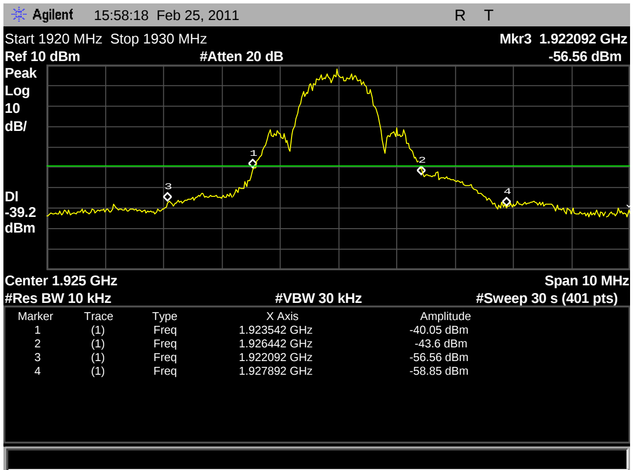
Fig. 20 - Spectrum analyzer screenshot for transmit emissions showing in-band unwanted emissions with the Base EUT transmitter at the middle carrier, 1924.992MHz, according to the requirements of 6.1.6.1.
