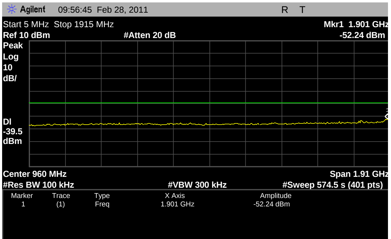
Fig. 31 – Base EUT out-of-band emissions showing the region from 5MHz to 1915MHz, with the transmitter using the highest carrier, 1928.448MHz.
