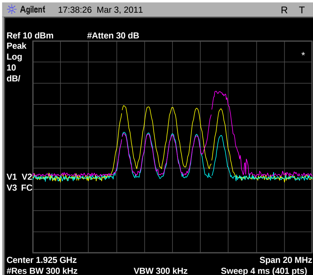
Fig. 43 - Emissions and interference profile spectrum, Base EUT, test 7.3.2.
