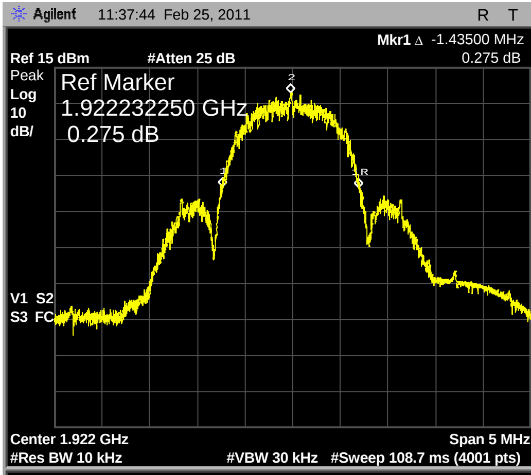
Fig. 10 - Base EUT, 1.45MHz emissions bandwidth on low carrier, 1.435 MHz.
