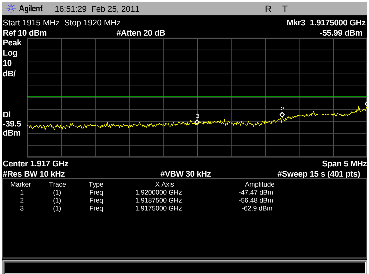
Fig. 24 – Base EUT out-of-band emissions showing the regions from band edge to -1.25MHz, and from -1.25MHz to -2.5MHz, with the Base EUT transmitting on the lowest carrier, 1921.536MHz. . Note the green display line is the spec limit marker only for the region outside +2.5MHz.
