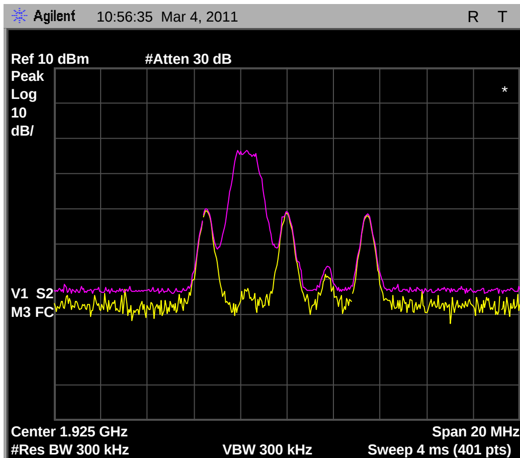
Fig. 46 - Emissions and interference profile spectrum, Base EUT, test 7.3.3(d).
