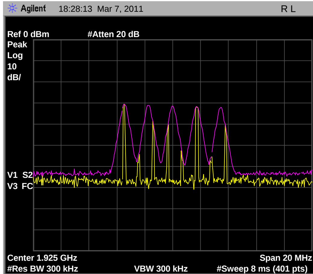
Fig. 52 - Base EUT shown deferring when all channels are blocked with 50uS pulses at T_U + U_M . Top (purple) trace is max hold showing interference only with no Base EUT RF transmissions. Bottom (yellow) trace is an instantaneous capture of individual pulses.
