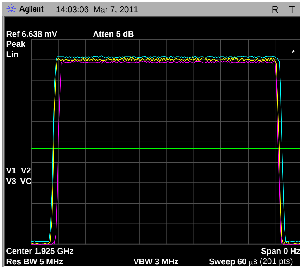
Fig. 51 – 50uS interference pulse for 7.5(c), duration and amplitude variation over the duration of the 50 uS pulse and over multiple pulses. Spectrum analyzer is set to linear response.
