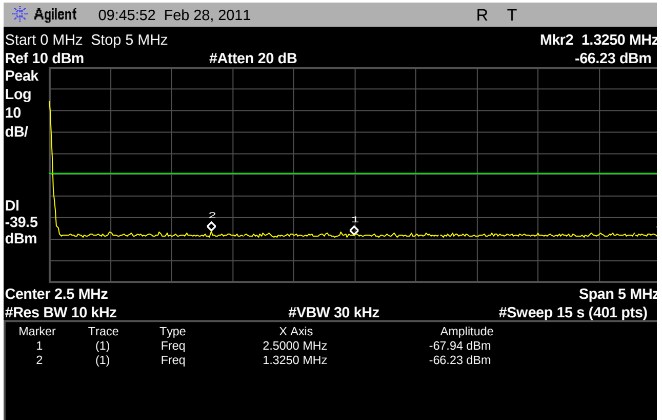
Fig. 30 – Base EUT out-of-band emissions showing the regions from DC to 5MHz, with the transmitter using the highest carrier, 1928.448MHz.
