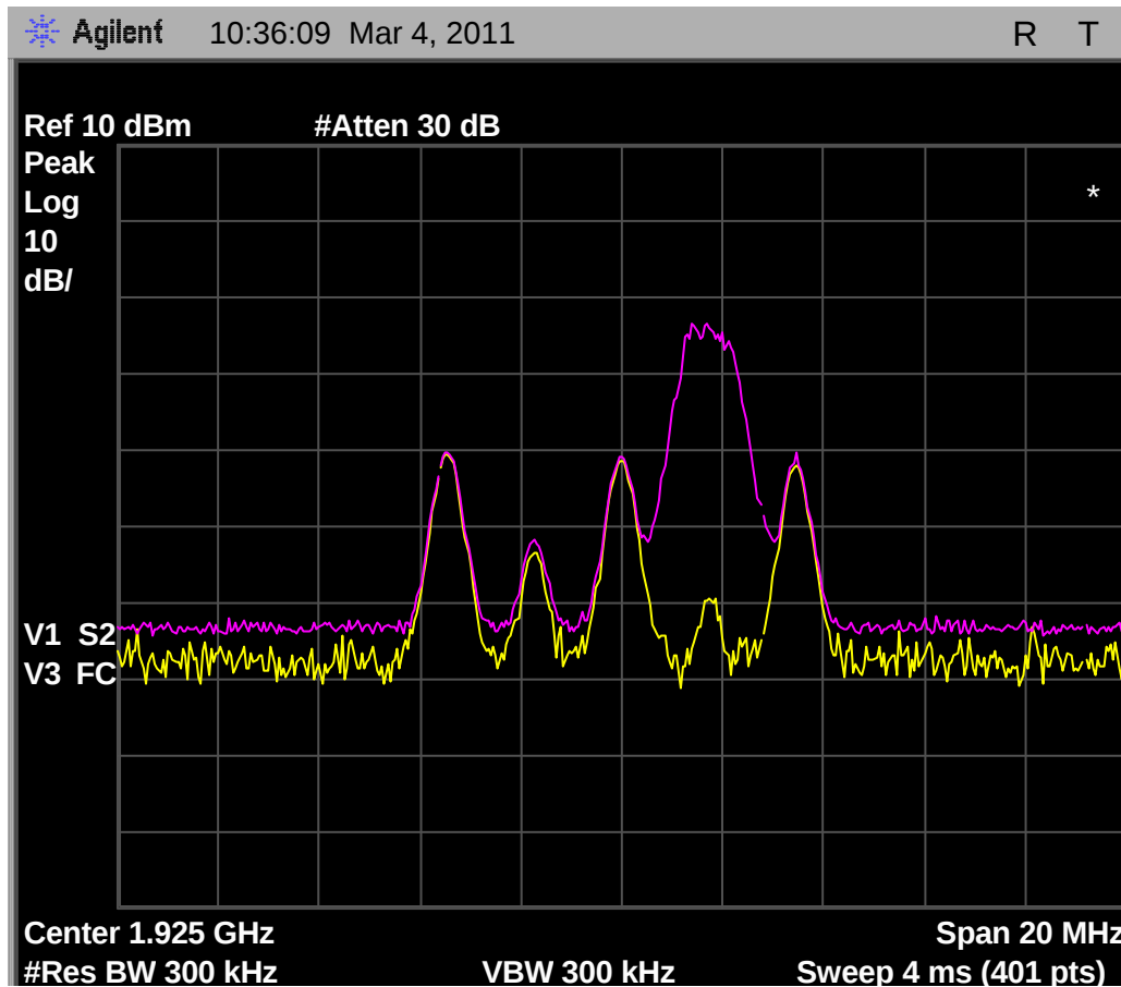
Fig. 45 - Emissions and interference profile spectrum, Base EUT, test 7.3.3(c).
