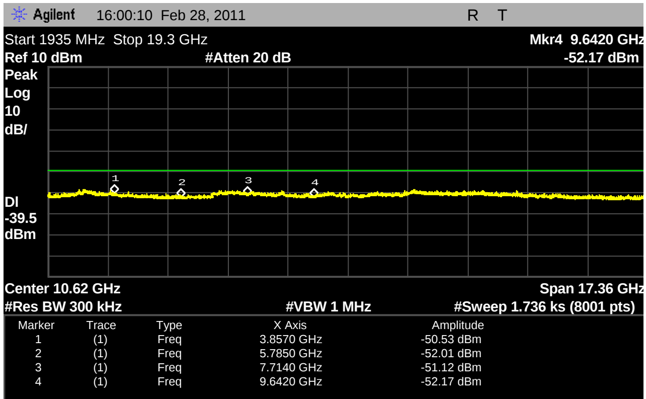
Fig. 71 - Base EUT in minimum power WBM on high carrier. All harmonics are below specification in minimum power, even when measured in the 300kHz (greater) resolution bandwidth.
