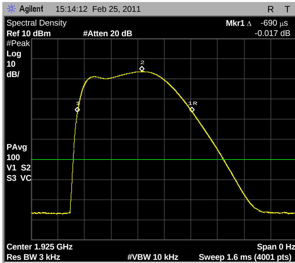
Fig. 15 – Zero-span sweep for Base EUT, middle carrier, for 3kHz maximum power spectral density. The peak level is at -6.47dBm, and the interval between samples at the -20dB points spans is 690.0us.
