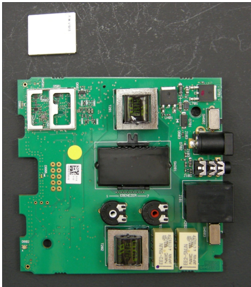
PCB Bottom – no shield
