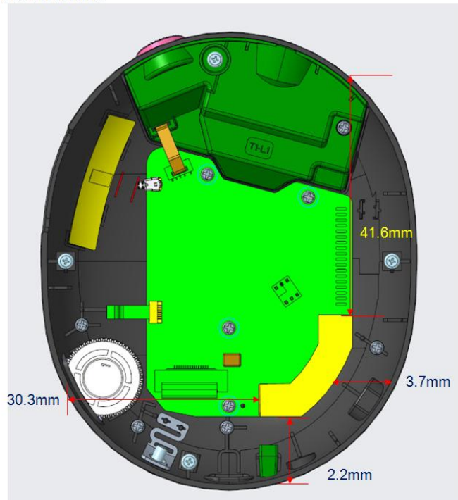
1571 PCB antenna
