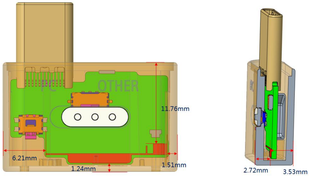
Dongle antenna
