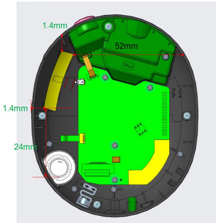
1577 FPC antenna
