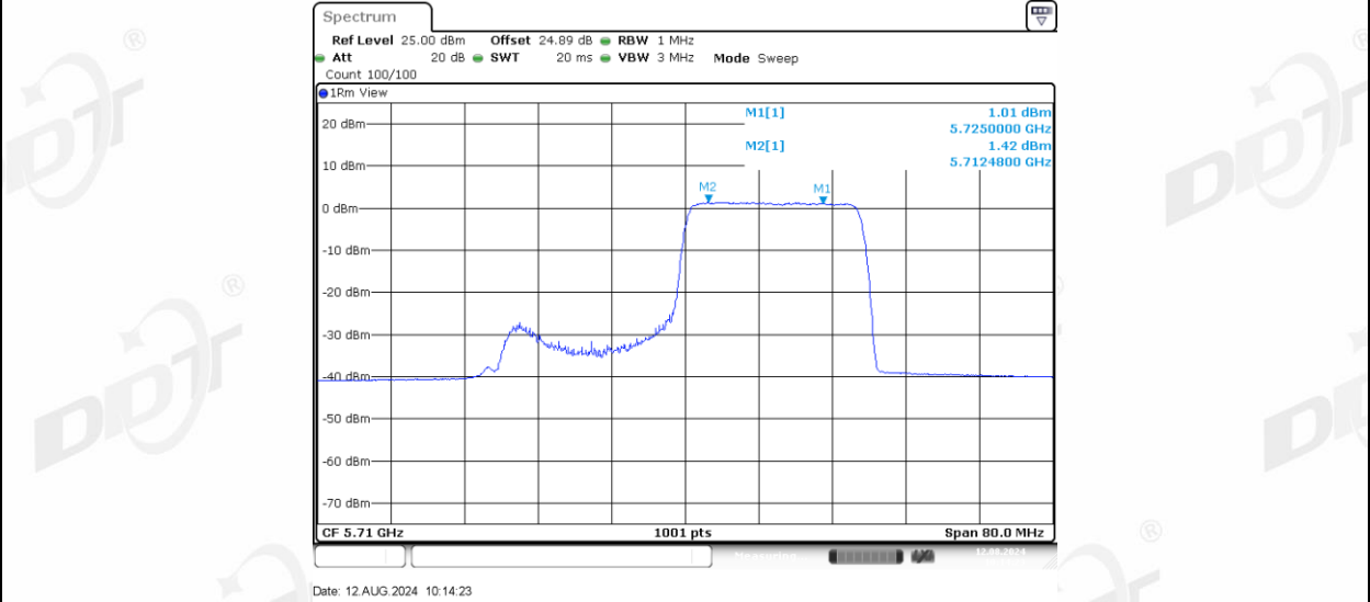
11AX40MIMO Ant-3_5710_UNII-2C_106Tone_RU53
