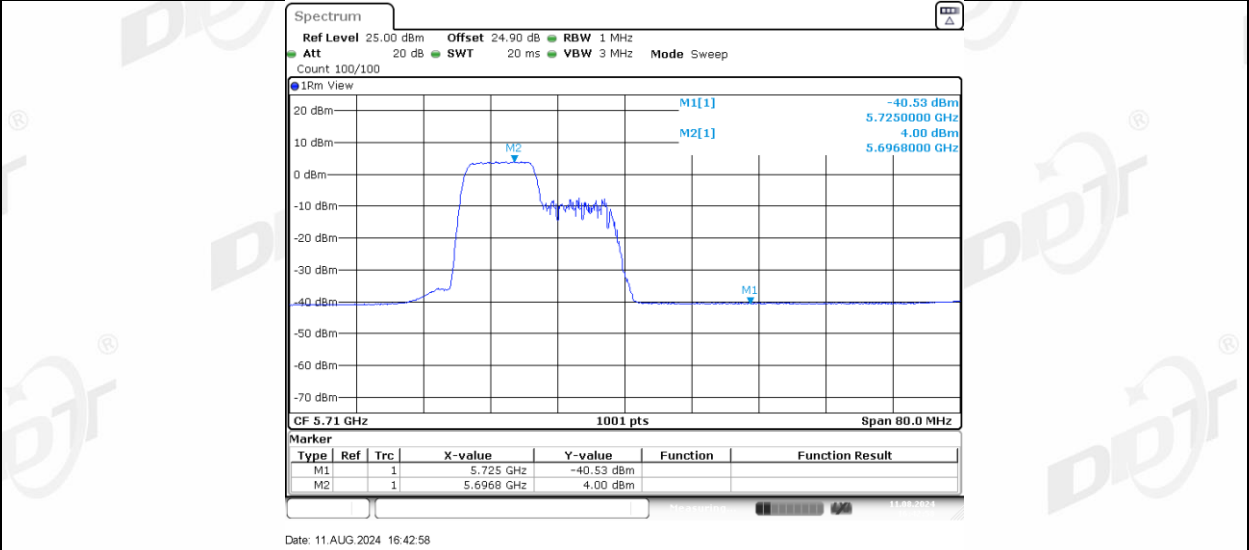
11AX40MIMO Ant-3_5710_UNII-2C_106Tone_RU56
