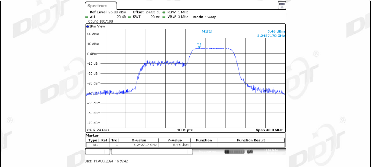
11AX20MIMO Ant-3 5240_26Tone_RU0
