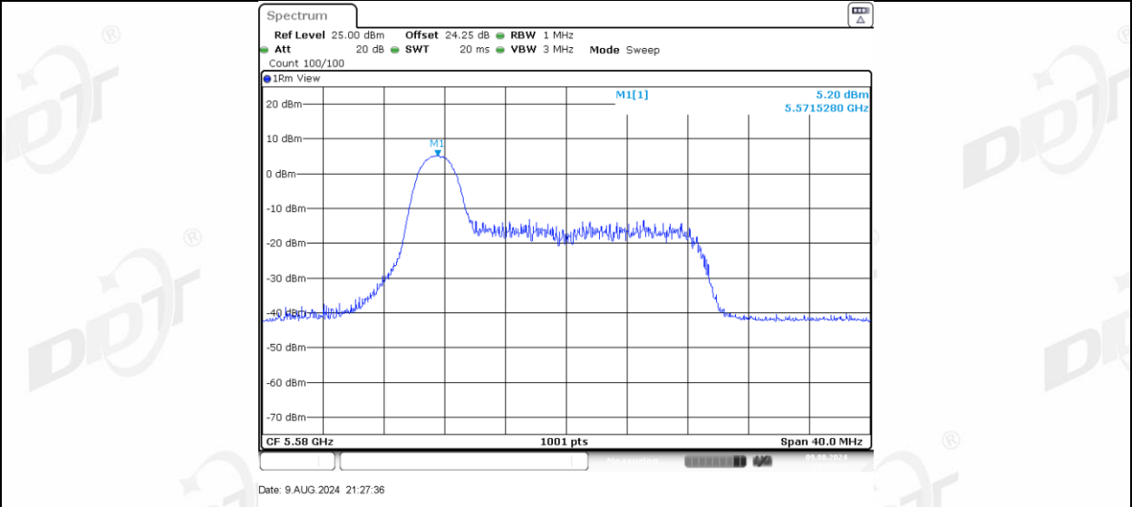
11AX20MIMO Ant-1_5580_26Tone_RU4
