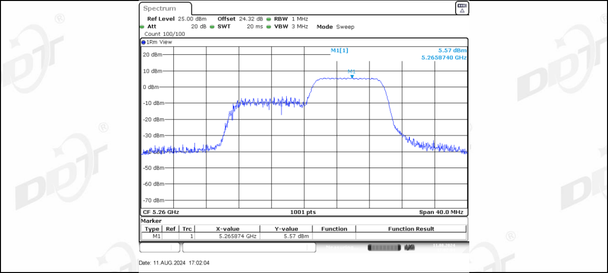
11AX20MIMO Ant-3 5260 26Tone RU0
