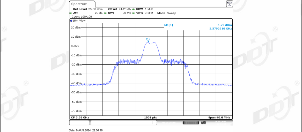
11AX20MIMO Ant-1_5580_26Tone_RU8
