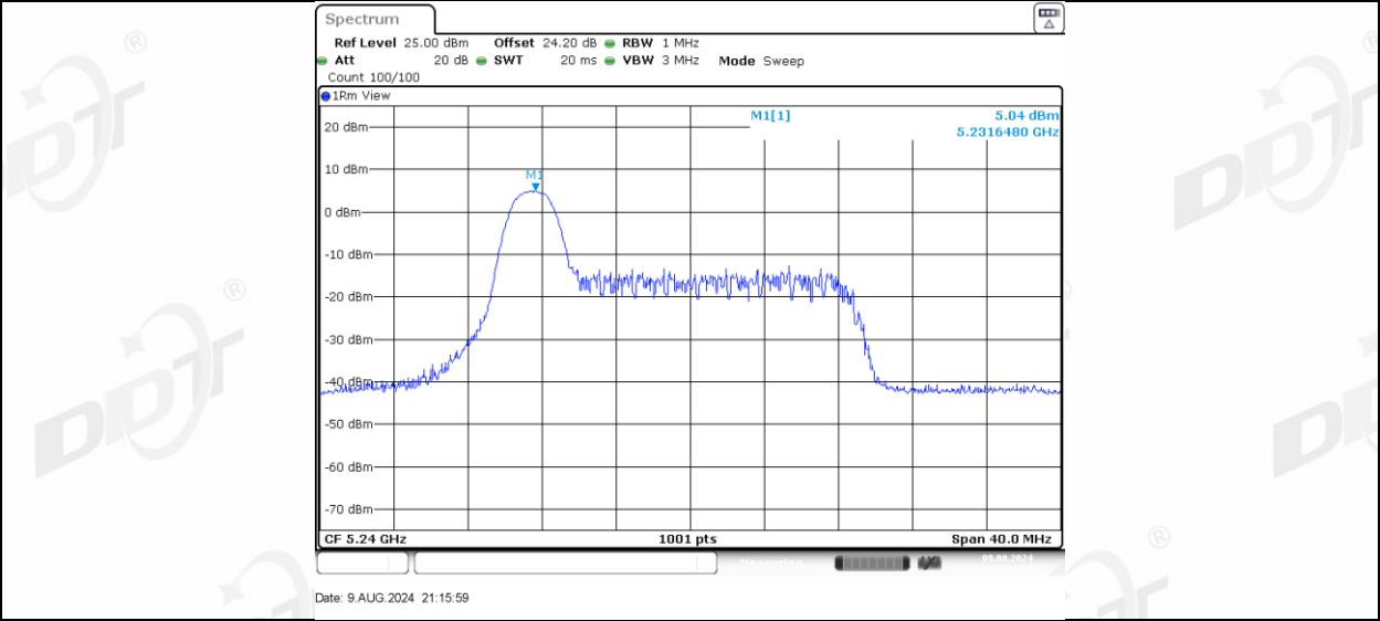
11AX20MIMO Ant-3 5240_26Tone_RU4
