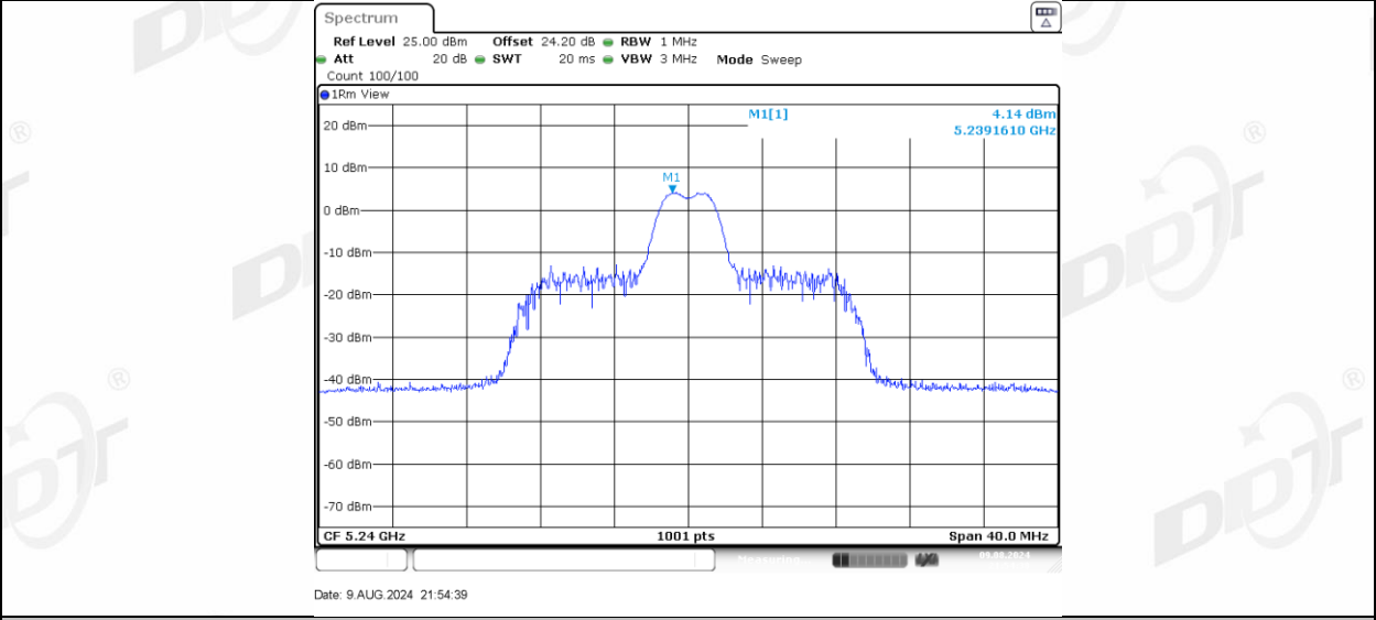
11AX20MIMO Ant-3 5240_26Tone_RU8
