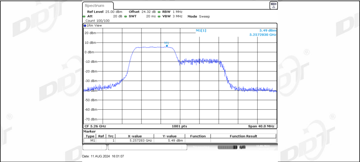
11AX20MIMO Ant-1 5260 106Tone RU54
