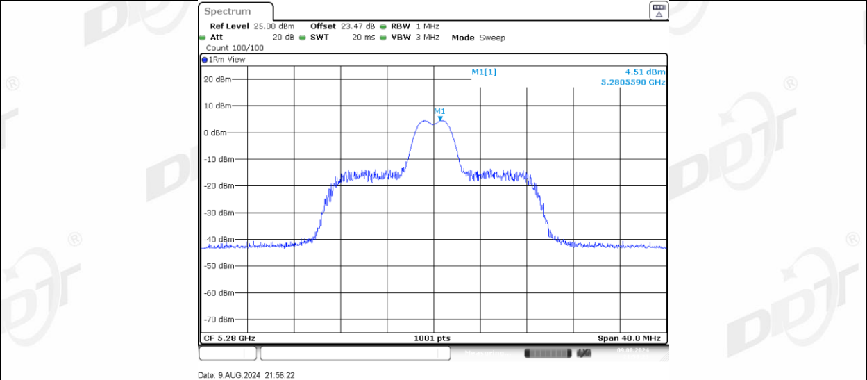
11AX20MIMO Ant-1_5280_26Tone_RU8
