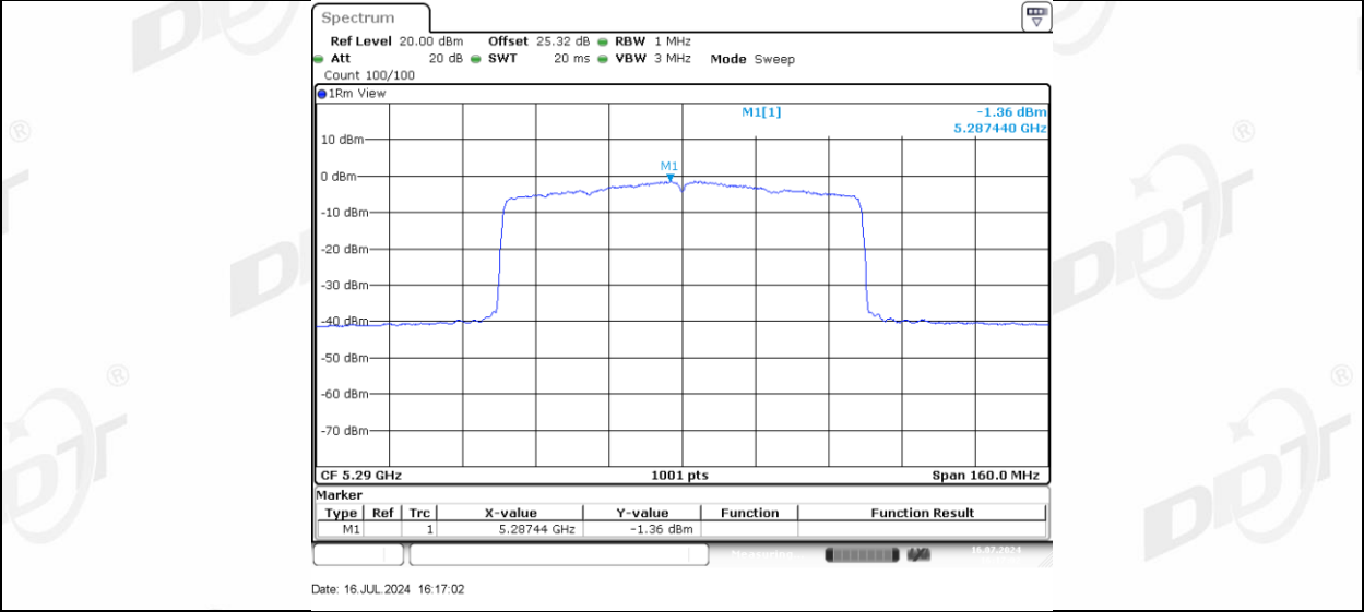
11AX80MIMO Ant-3_5290
