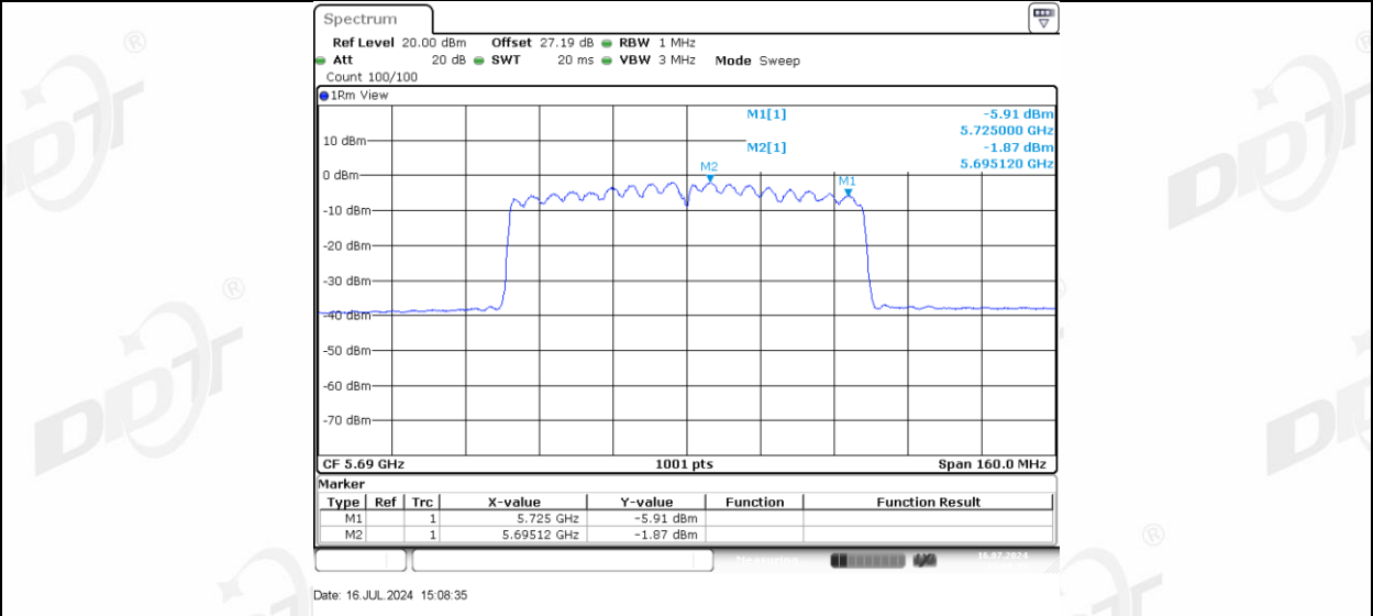
11AC80MIMO Ant-3_5690_UNII-2C
