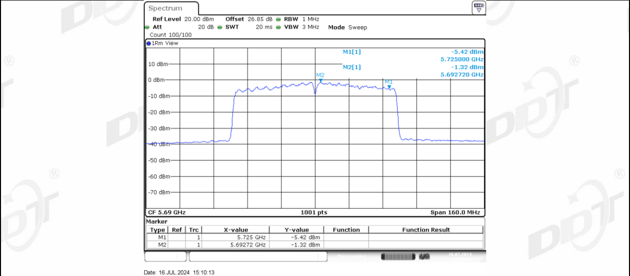
11AC80MIMO Ant-1_5690_UNII-3
