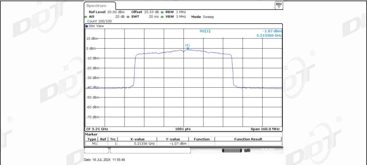
11AX80MIMO Ant-3_5210
