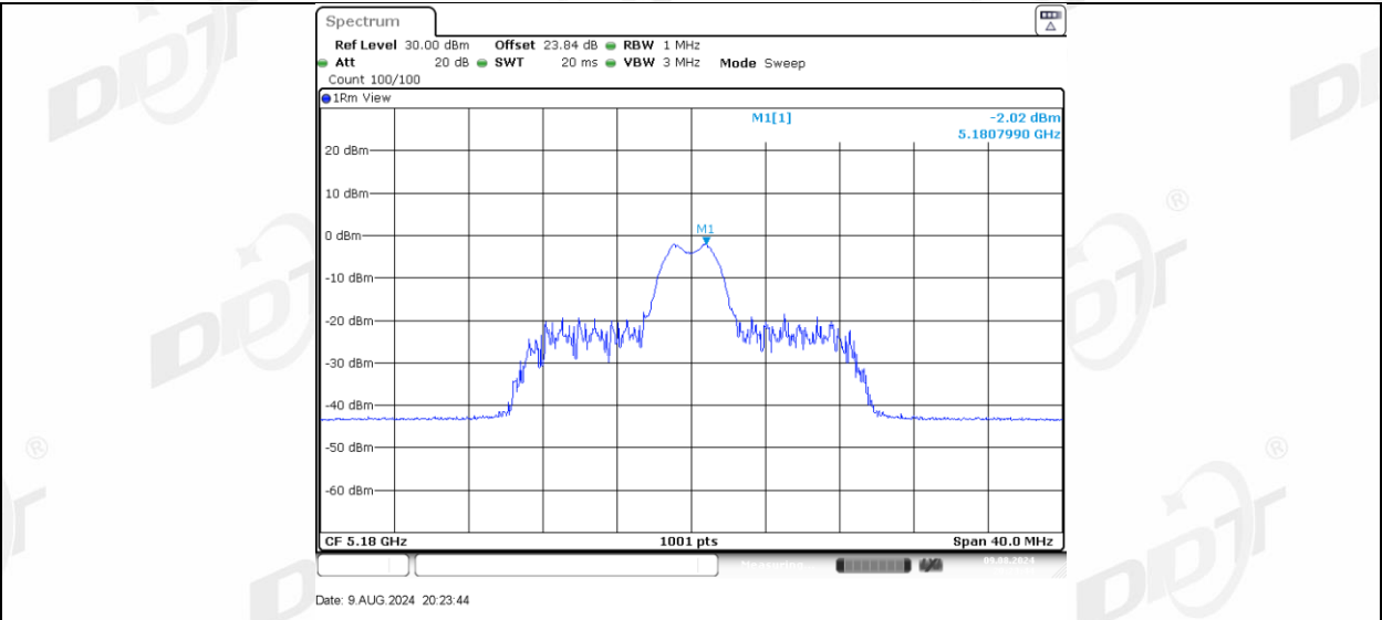
11AX20MIMO Ant-1 5180_26Tone_RU8
