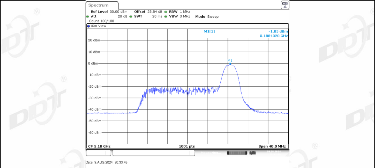
11AX20MIMO Ant-1 5180_52Tone_RU37
