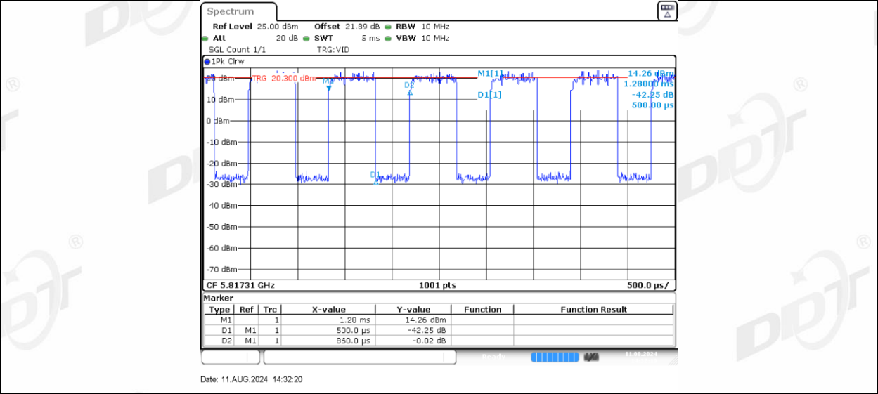
11AX20MIMO Ant-3 5825 52Tone RU39
