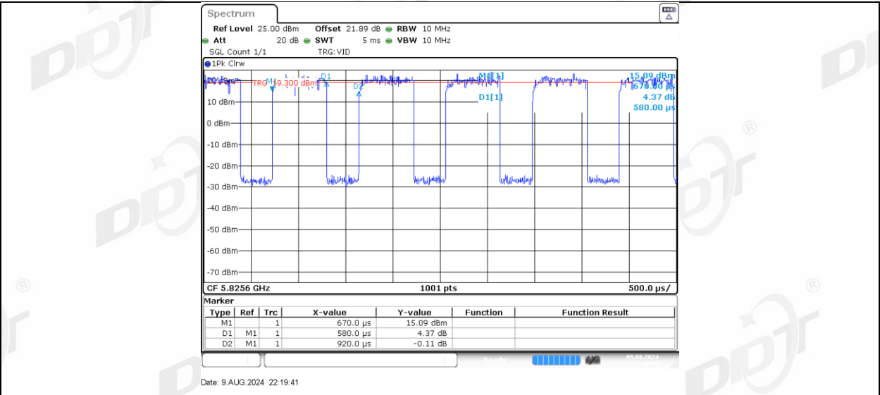
11AX20MIMO Ant-3 5825 26Tone RU8
