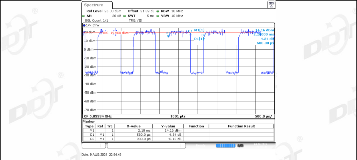
11AX20MIMO Ant-3 5825 52Tone RU37
