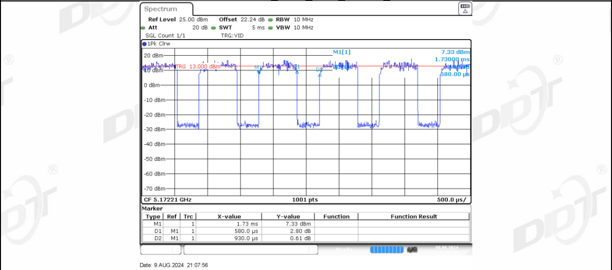
11AX20MIMO Ant-3_5180_26Tone_RU4
