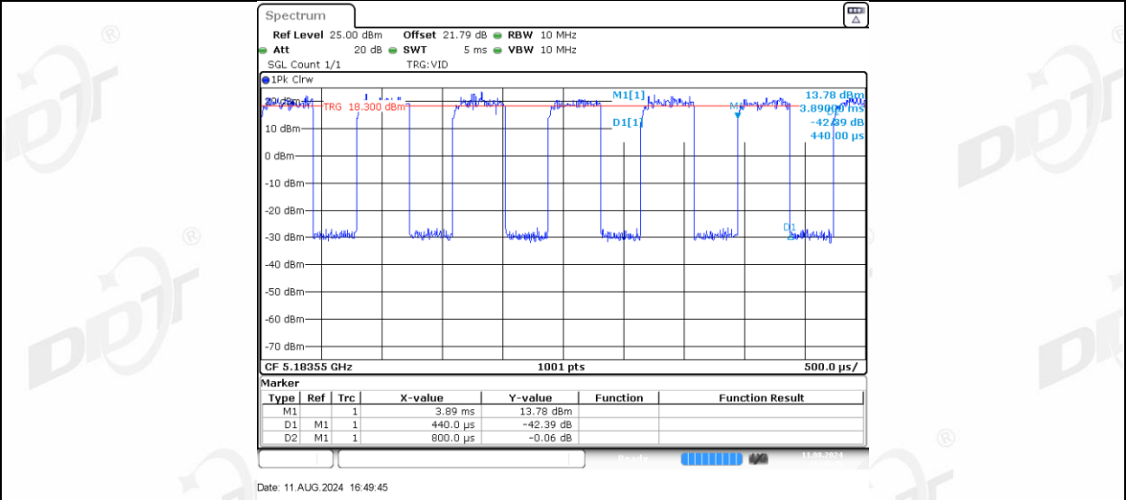
11AX20MIMO Ant-3_5180_26Tone_RU0
