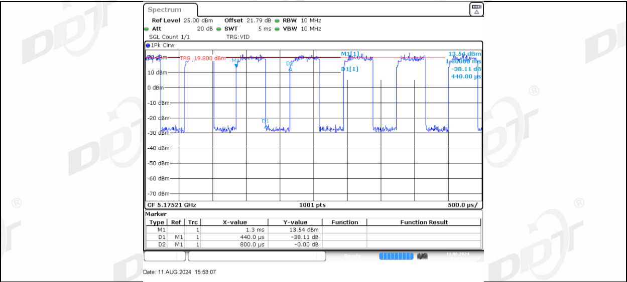
11AX20MIMO Ant-1_5180_106Tone_RU54
