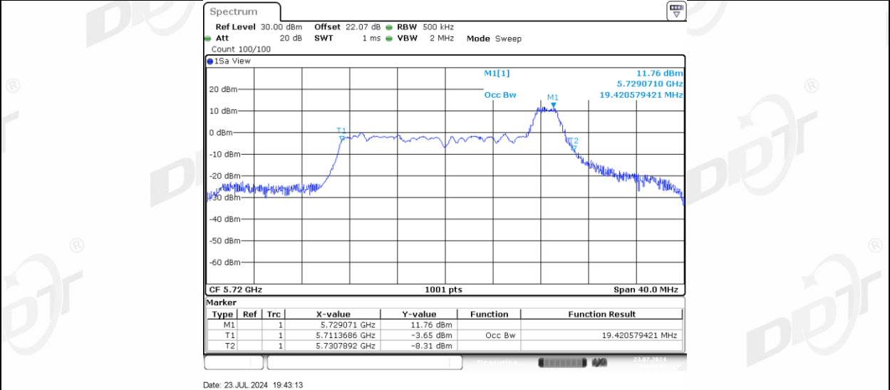
11AX20MIMO Ant-1_5720_52Tone_RU37
