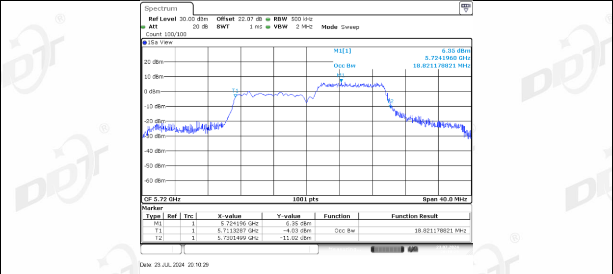
11AX20MIMO Ant-3_5720_26Tone_RU0
