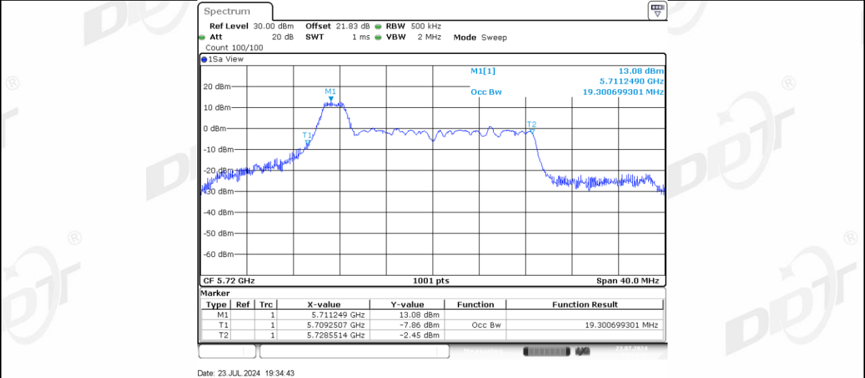
11AX20MIMO Ant-3_5720_26Tone_RU4
