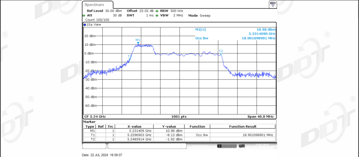
11AX20MIMO Ant-1 5240_52Tone_RU39
