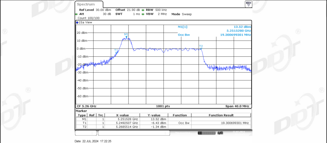
11AX20MIMO Ant-3 5260 26Tone RU4
