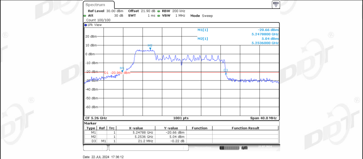
11AX20MIMO Ant-3 5260_52Tone_RU39
