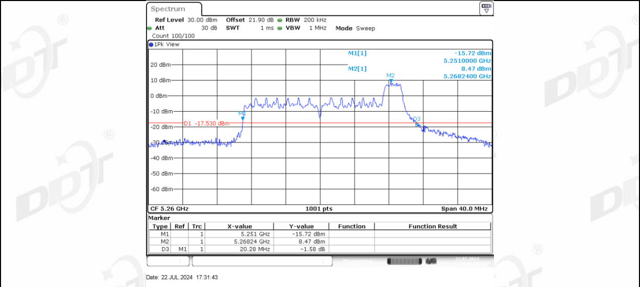
11AX20MIMO Ant-3 5260_52Tone_RU37
