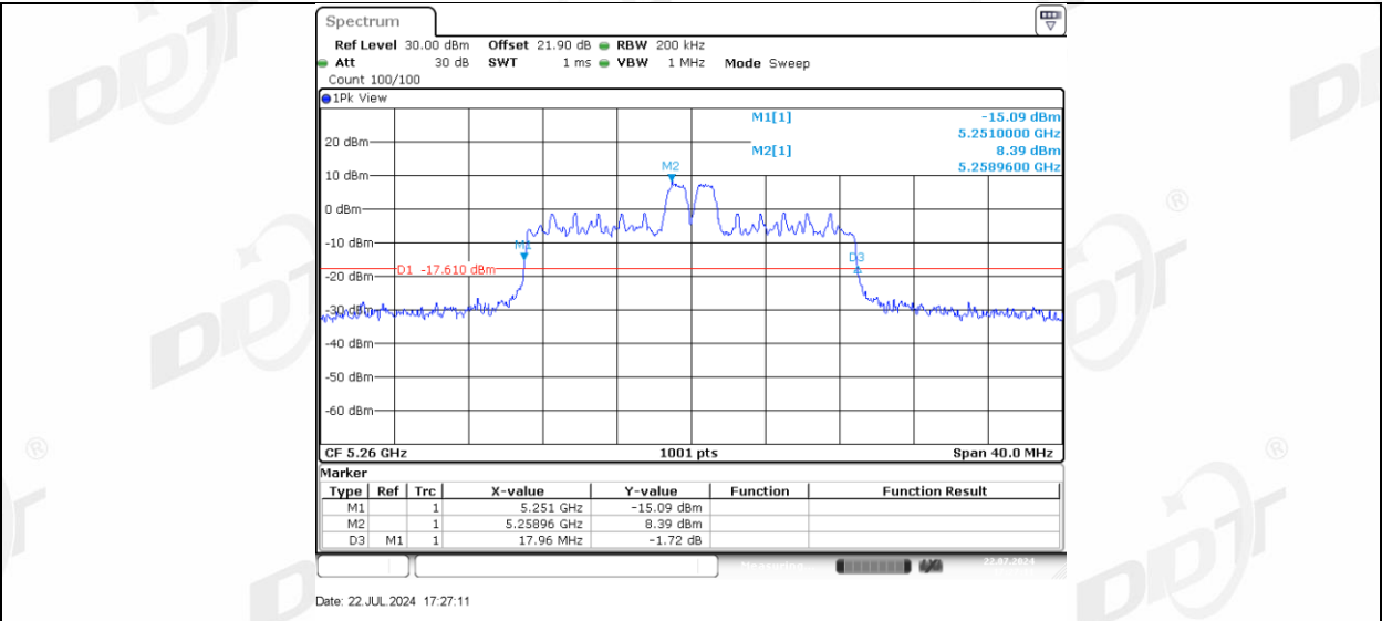
11AX20MIMO Ant-3 5260_26Tone_RU8
