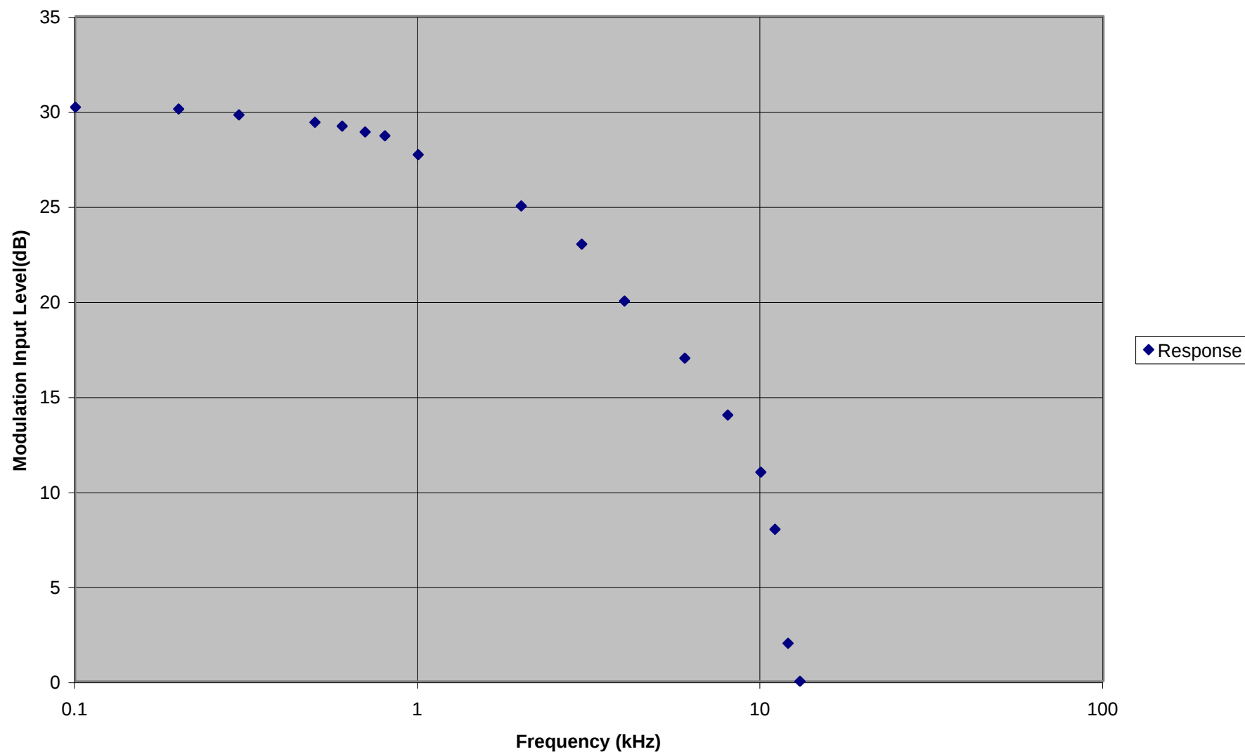
Frequency Response
