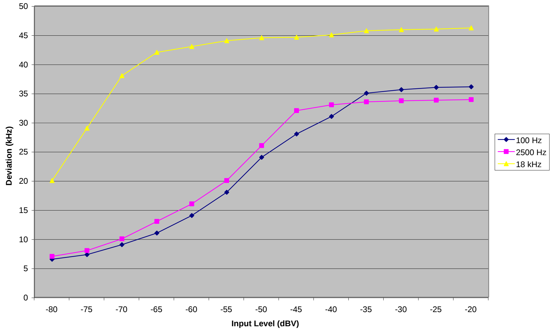
Modulation Characteristics
