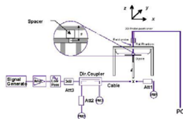
Figure 12-1 System Verification Setup Diagram
