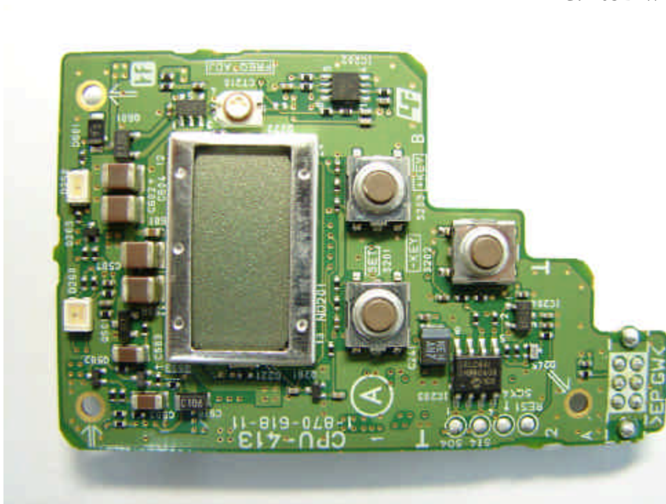
CPU Side A
