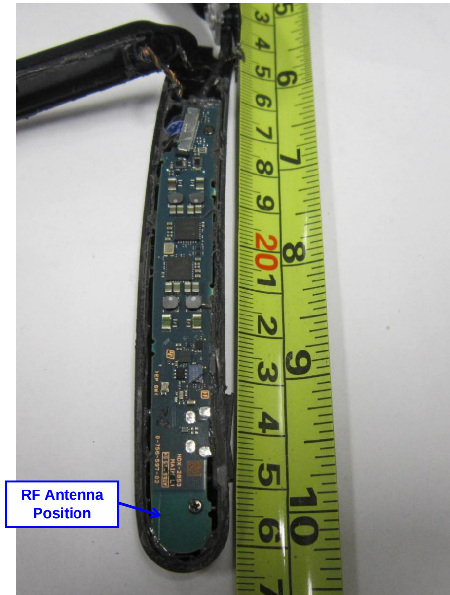
Main-Board PCB Component View
