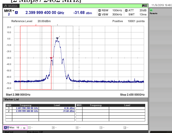
[2 Mbps / 2402 MHz]
