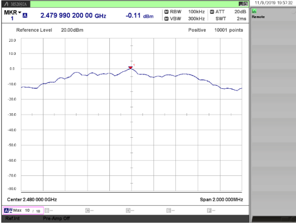
[2 Mbps / 2480 MHz]
