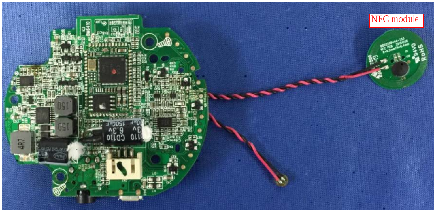
Main board
