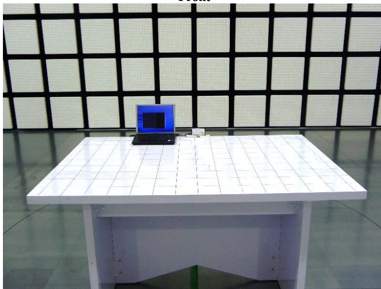
Loop antenna: Horizontal
