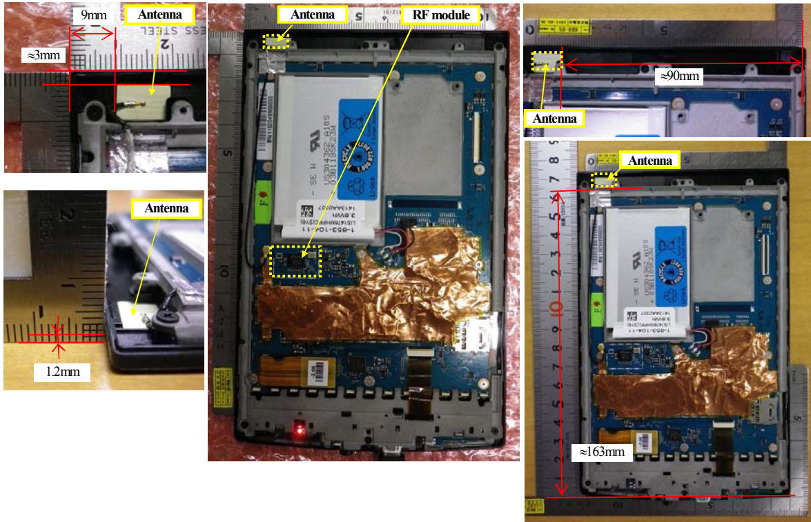
[Antenna position / dimension on the drawing]
