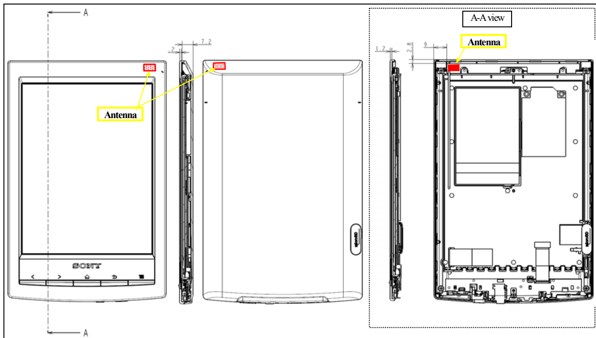
[Antenna position / dimension on the drawing]
