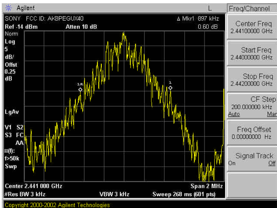
Plot A-2. 20dB Bandwidth Plot – Ch. 06
