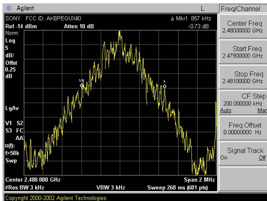
Plot A-3. 20dB Bandwidth Plot – Ch. 11
