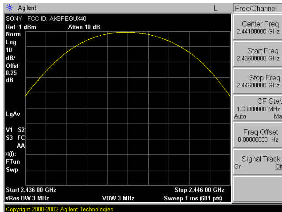
Plot A-5. Max. Peak Output Power Plot – Ch. 06
