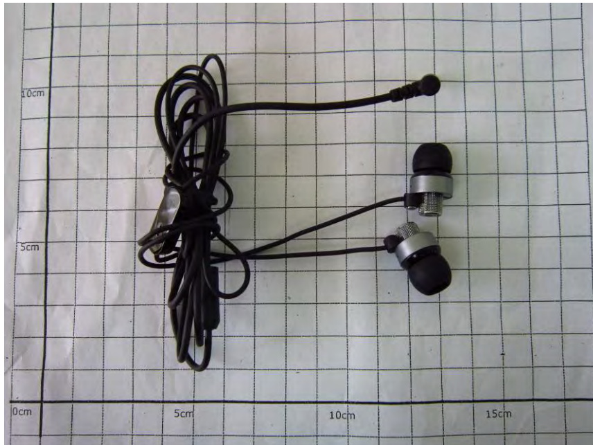
Fig.15 Headset (PCH-ZHS1 G)
