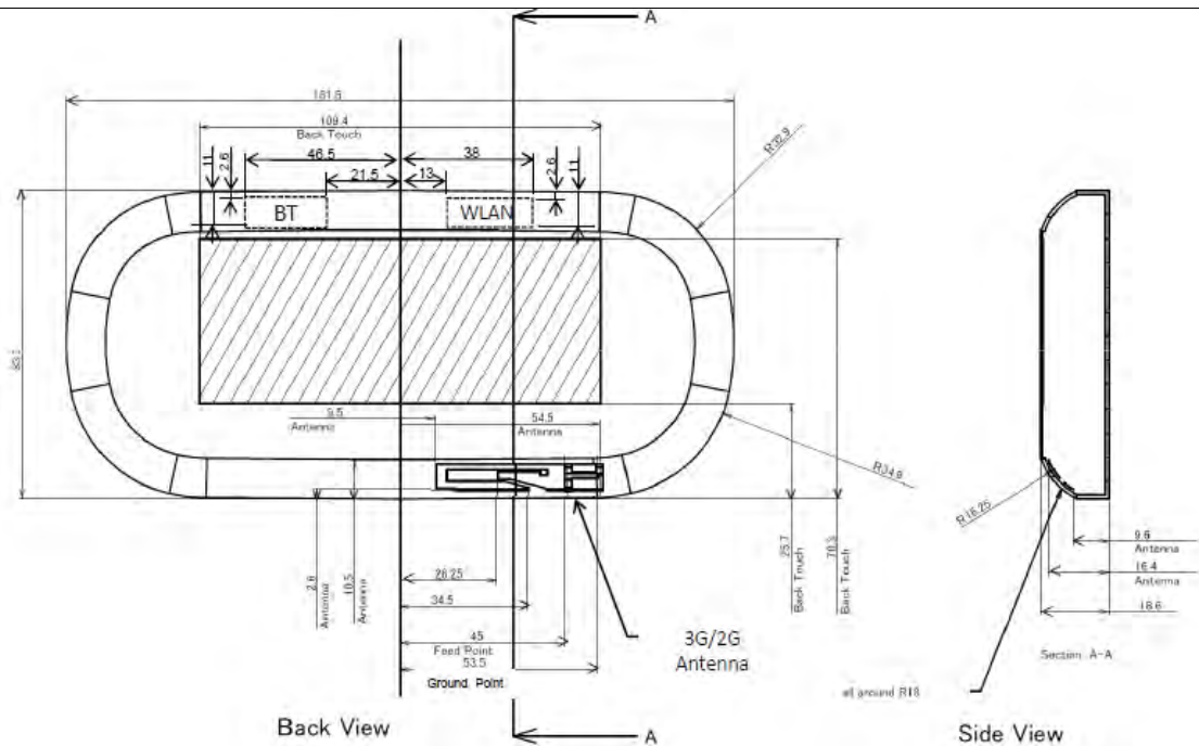
Fig.17 Antenna position of EUT
