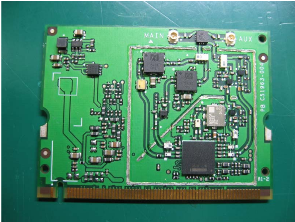
Wireless LAN Module front side without shielding
