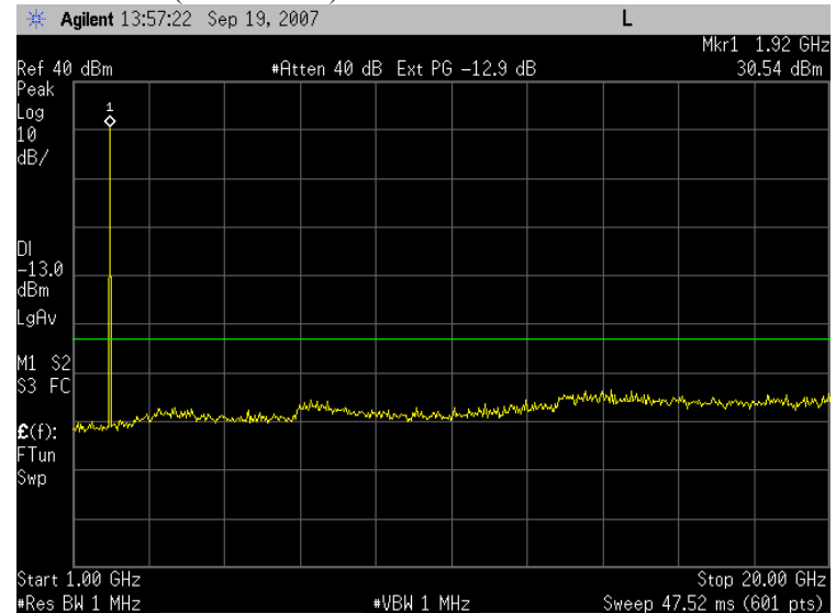
Plot 7.2 - 12 (GSM Ch810)
