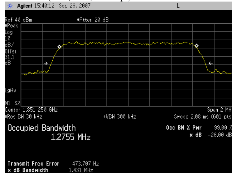
Plot 5.2 - 34 (Ch25, Rel 0, 153.6kbps)
