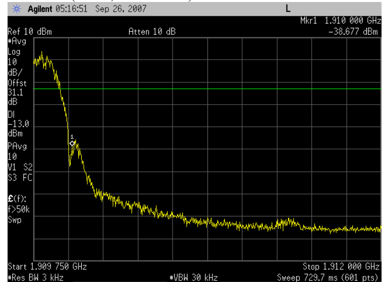
Plot 6.2 - 8 (Ch810, EGPRS 1900)
