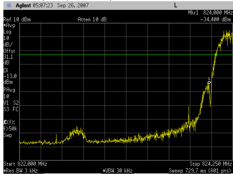
Plot 6.2 - 5 (Ch128, EGPRS 850)
