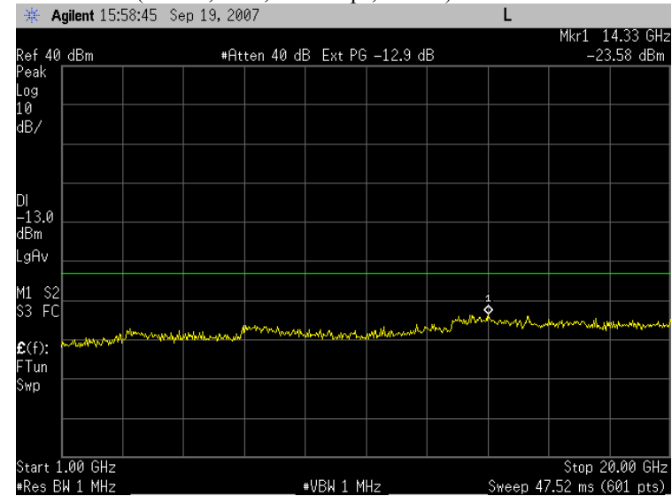
Plot 7.2 - 40 (EVDO, Rel0, 153.6kbps, Ch384)
