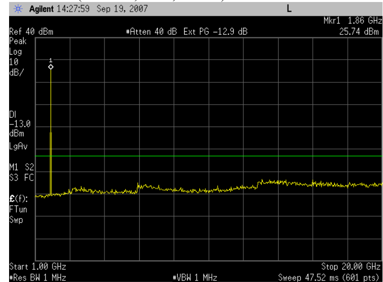
Plot 7.2 - 32 (WCDMA, Rel99, Ch9262)
