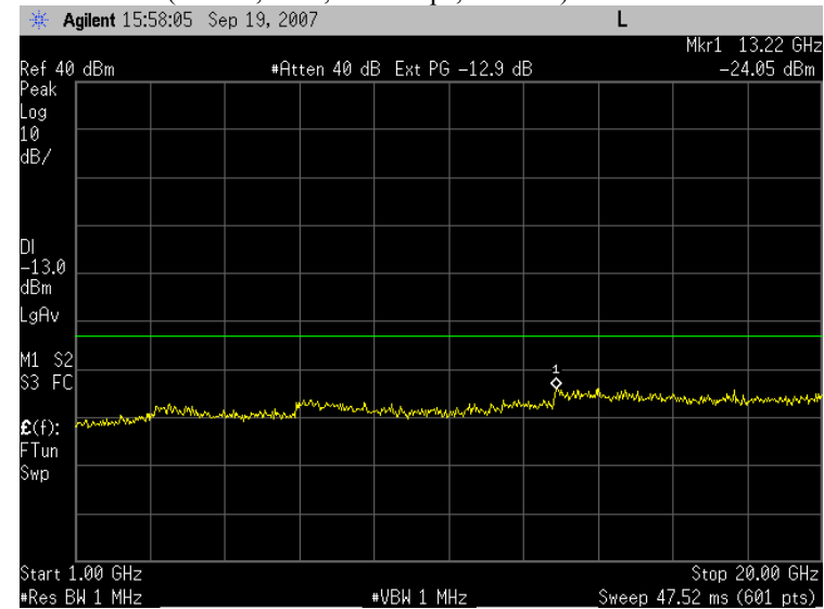
Plot 7.2 - 38 (EVDO, Rel0, 153.6kbps, Ch1013)
