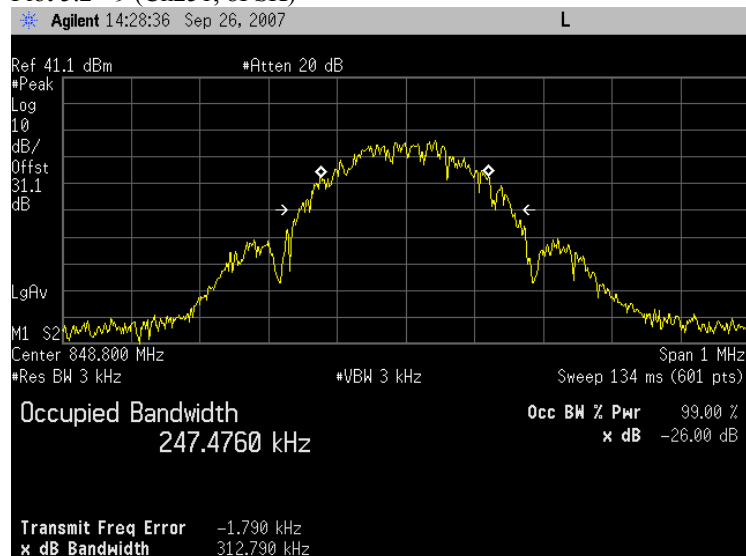
Plot 5.2 - 9 (Ch251, 8PSK)
