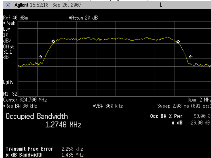
Plot 5.2 - 37 (Ch1013, Rel A, 4096 payload size)
