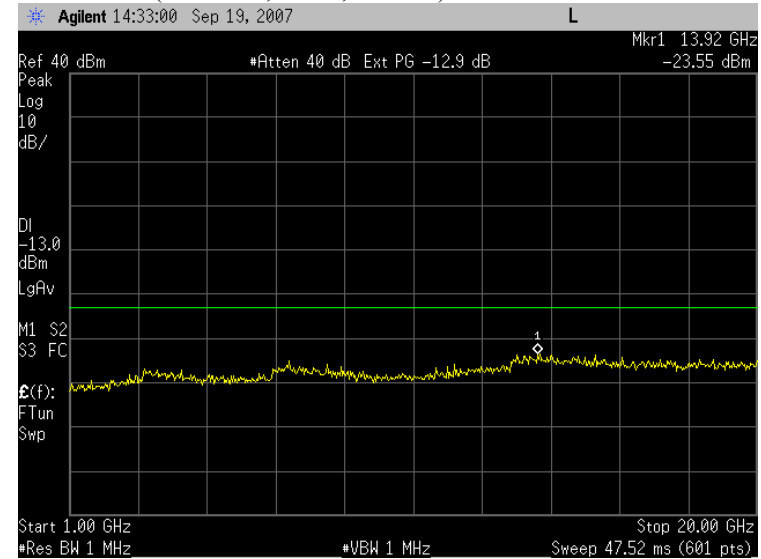
Plot 7.2 - 28 (WCDMA, Rel99, Ch4182)
