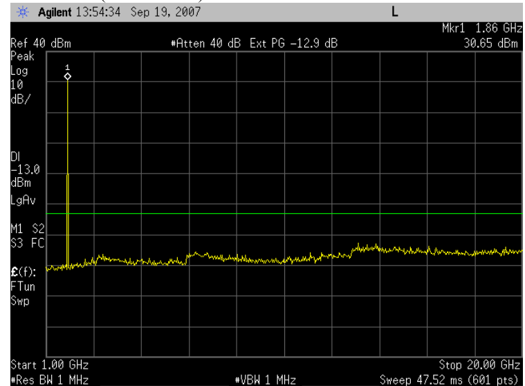
Plot 7.2 - 8 (GSM Ch512)
