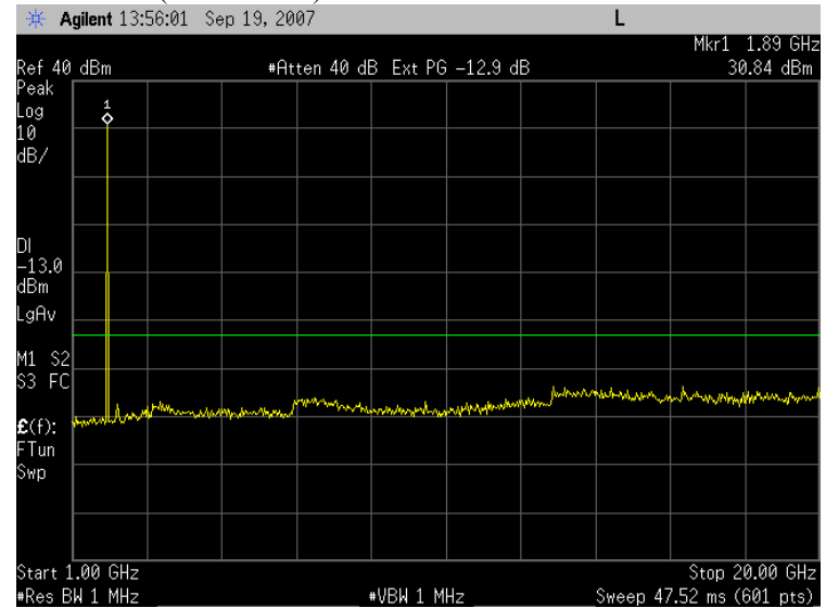
Plot 7.2 - 10 (GSM Ch661)
