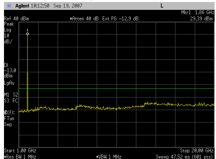
Plot 7.2 - 20 (EGPRS Ch512)
