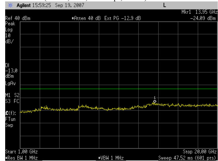
Plot 7.2 - 42 (EVDO, Rel0, 153.6kbps, Ch777)
