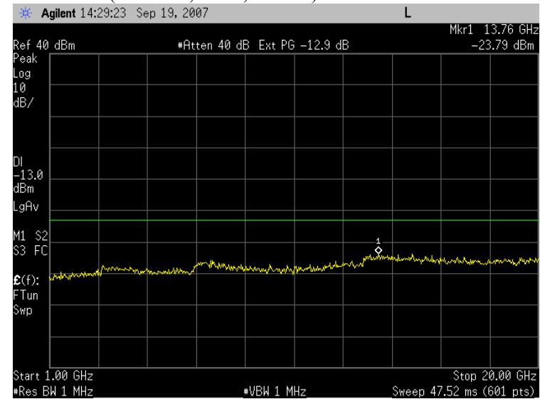
Plot 7.2 - 30 (WCDMA, Rel99, Ch4233)
