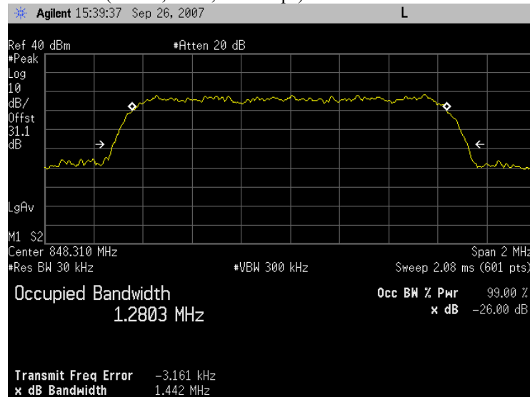
Plot 5.2 - 33 (Ch777, Rel 0, 153.6kbps)
