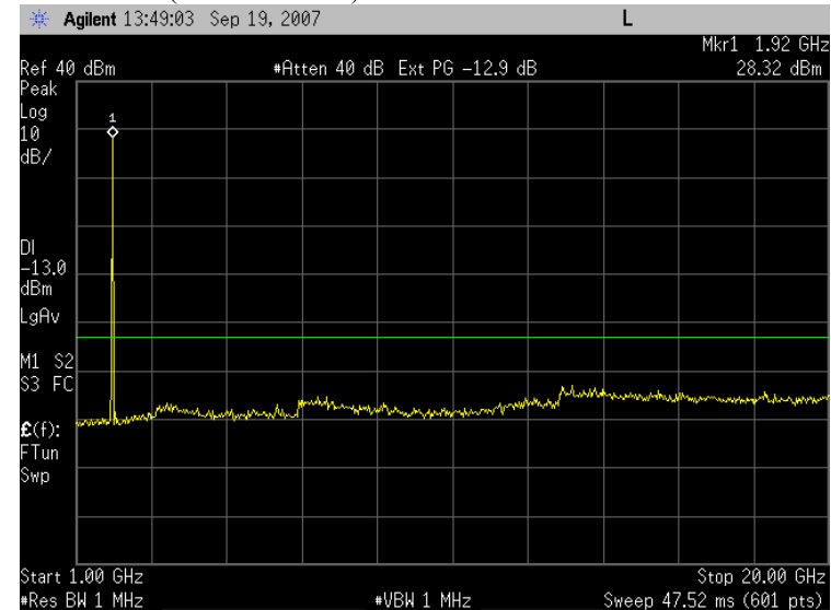
Plot 7.2 - 24 (EGPRS Ch810)
