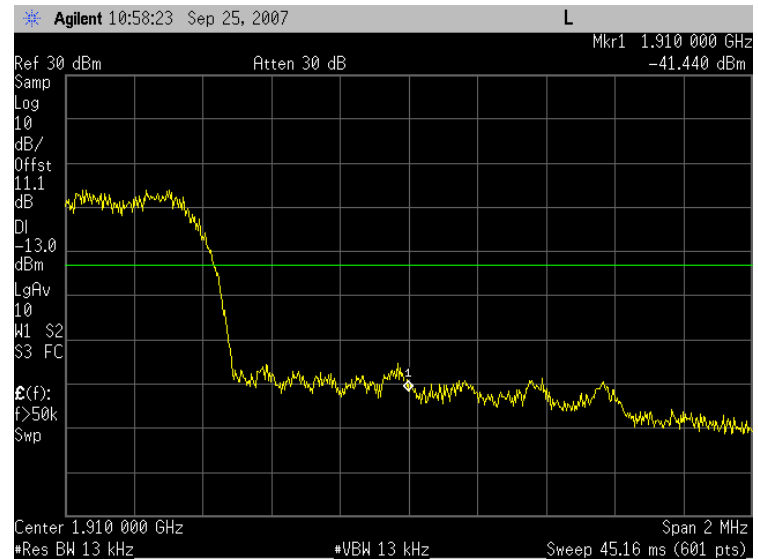
Plot 6.2 - 20 (Ch1175, 1x RC3 SO55)
