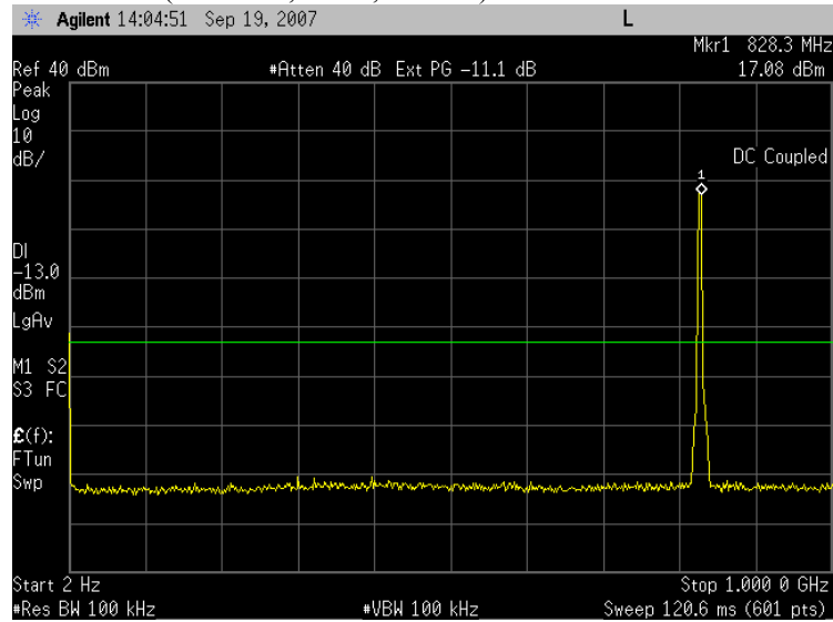
Plot 7.2 - 25 (WCDMA, Rel99, Ch4132)
