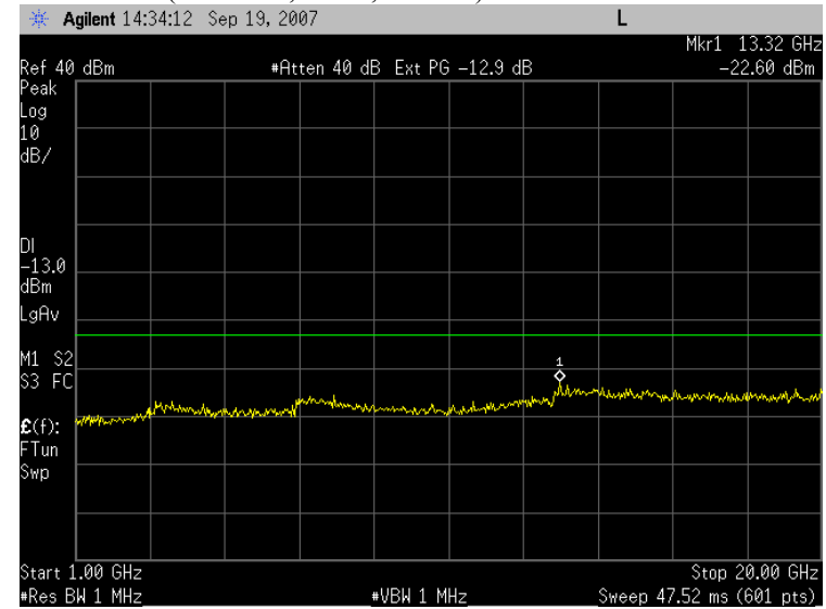
Plot 7.2 - 26 (WCDMA, Rel99, Ch4132)
