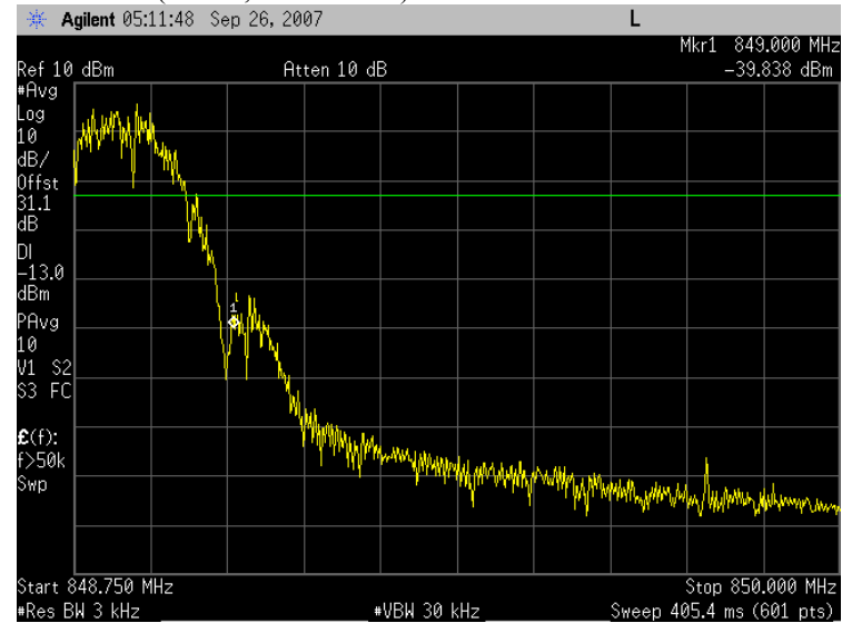
Plot 6.2 - 6 (Ch251, EGPRS 850)
