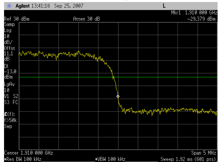
Plot 6.2 - 12 (Ch9538, WCDMA Rel 99)
