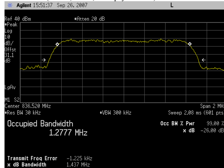
Plot 5.2 - 38 (Ch384, Rel A, 4096 payload size)
