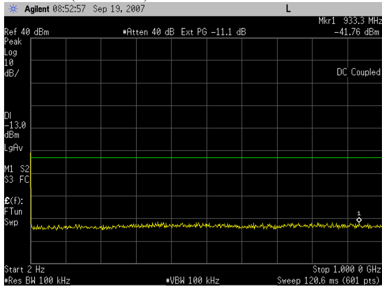
Plot 7.2 - 9 (GSM Ch661)
