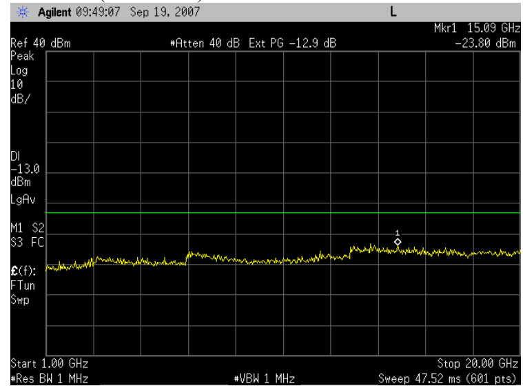
Plot 7.2 - 6 (GSM Ch251)
