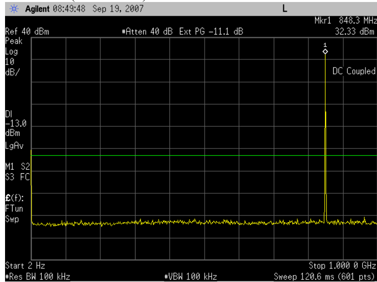
Plot 7.2 - 5 (GSM Ch251)
