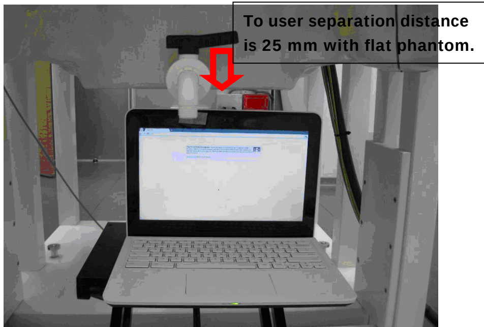
Fig.5 Top of LCD display mode
