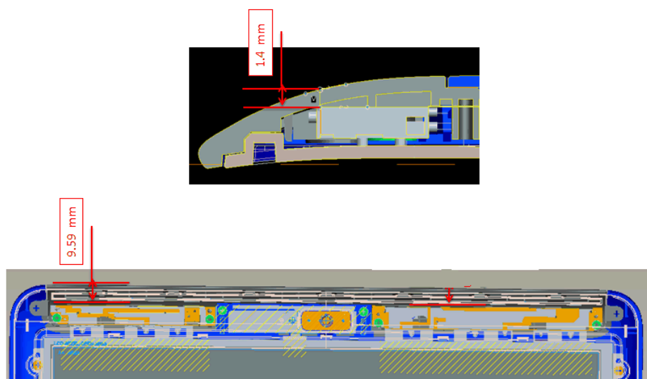
Fig.10 Antenna position of EUT
