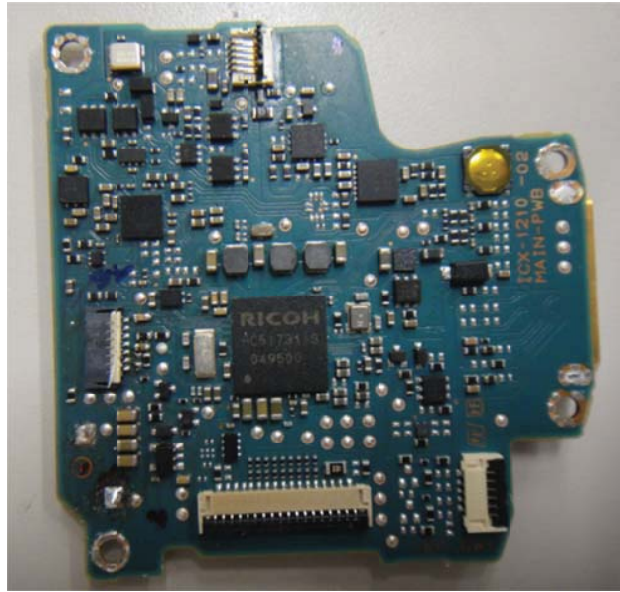
Main Board(Top)
