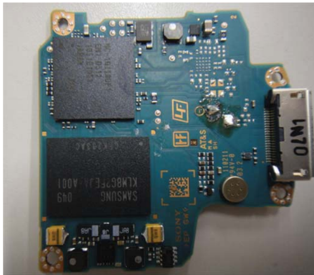
Main Board(Bottom)
