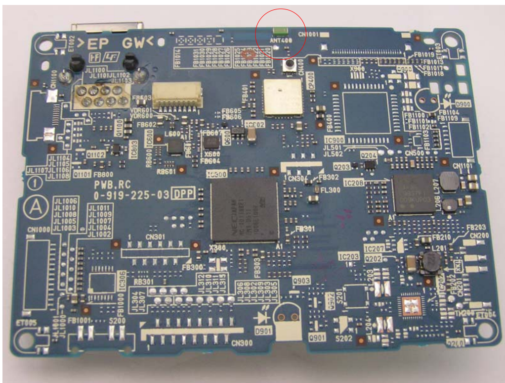
Antenna Part
