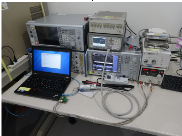
Maximum Conducted Output Power
