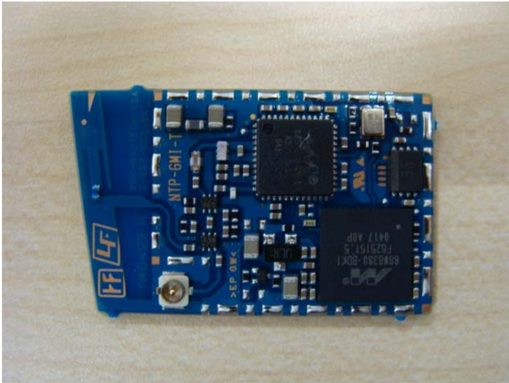
RF Module without shield (Front)
