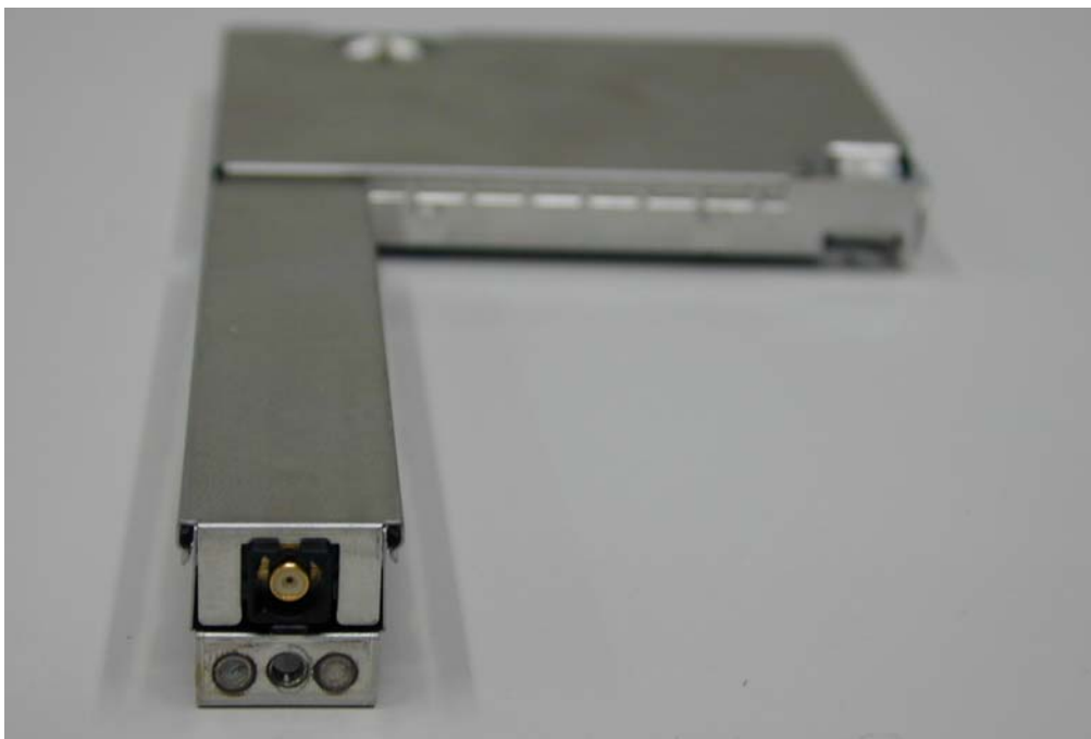
Front View of RF Connector with Shielding
