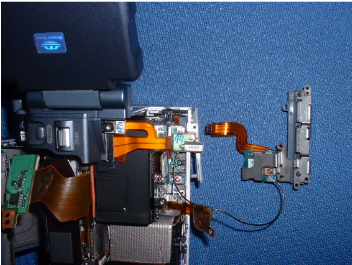
Antenna and Circuit board (connected) No.2
