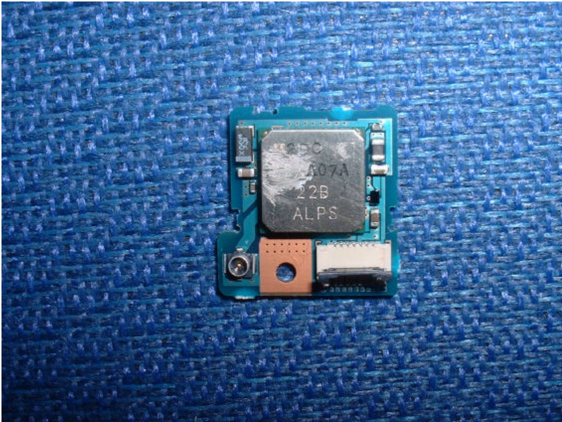
Circuit board with shield (front)
