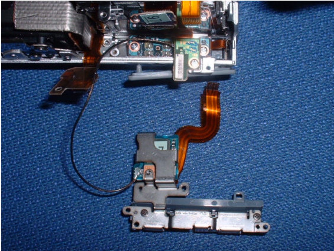
Antenna and Circuit board (connected)
