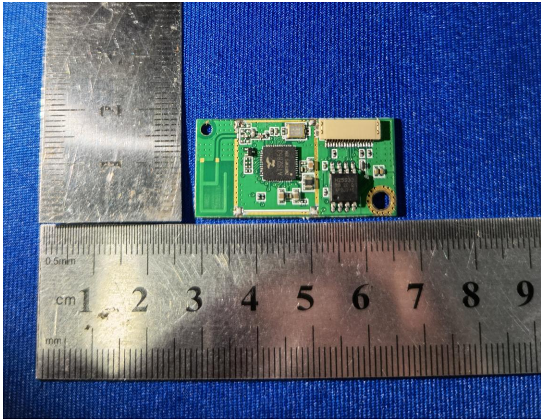
Figure 3 Inside of the EUT
