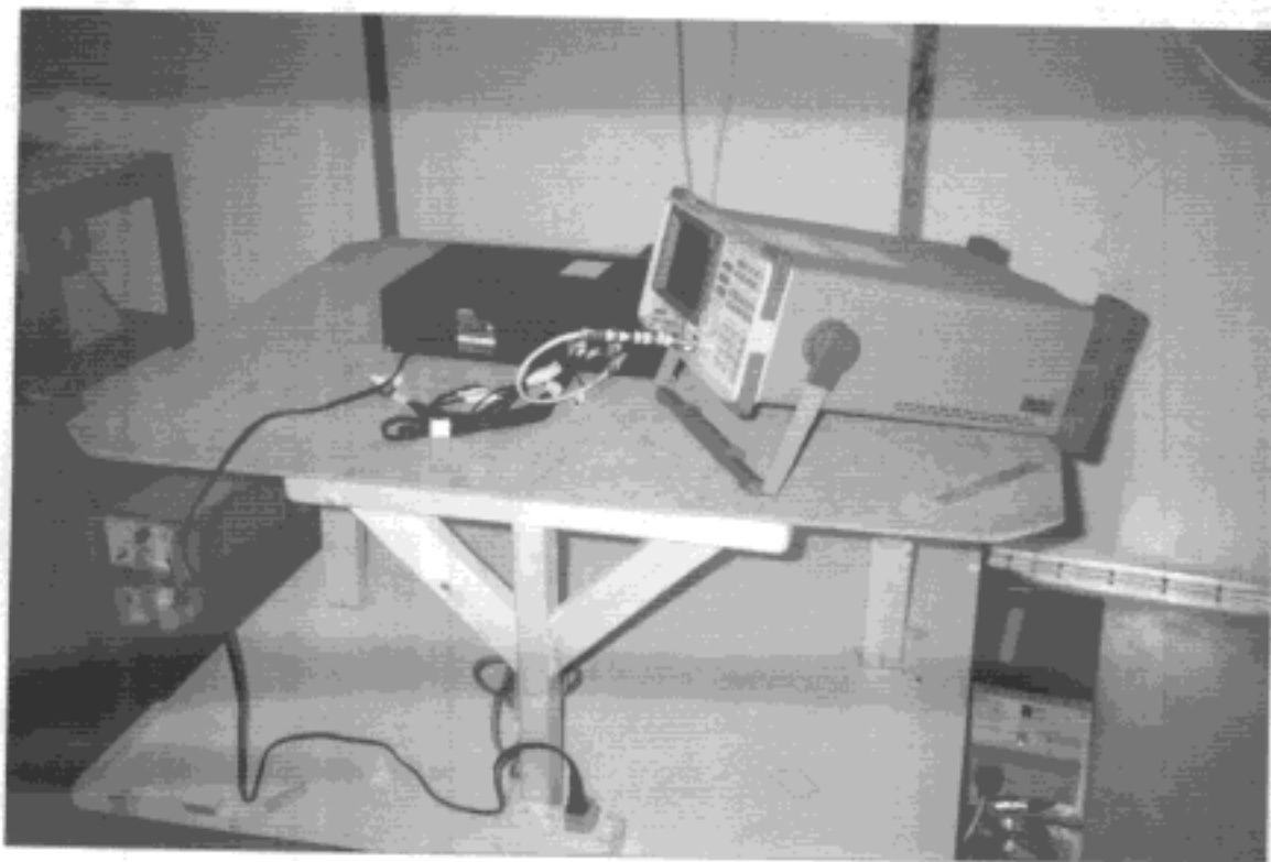
Output Terminal Conducted Spurious Emission Test Setup
