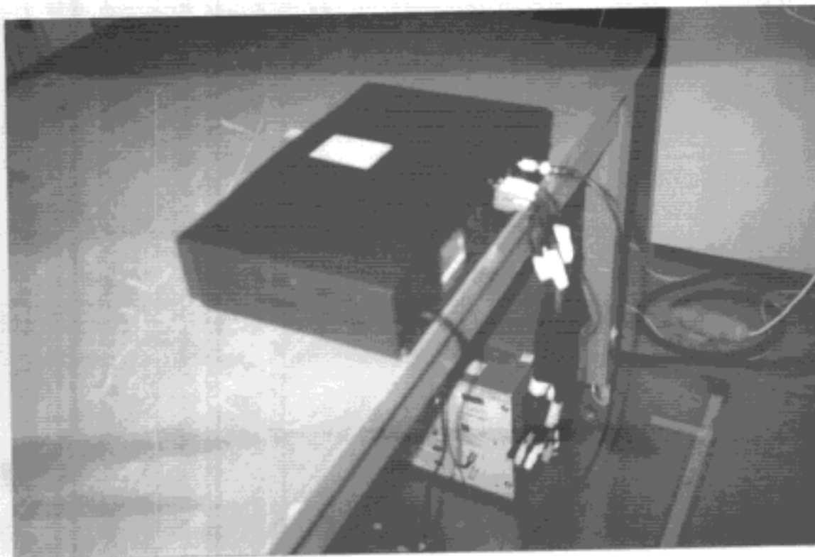
Conducted emission test setup (back view)
