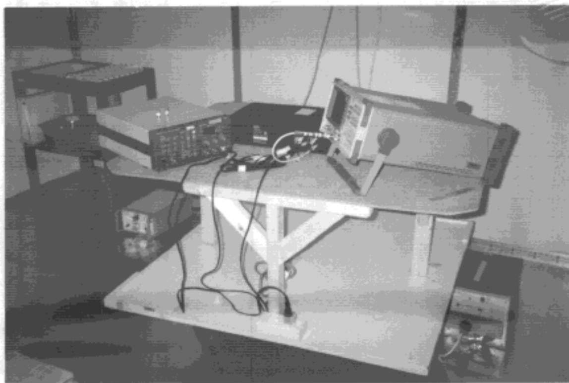
Output Signal Level Measurement Test Setup
