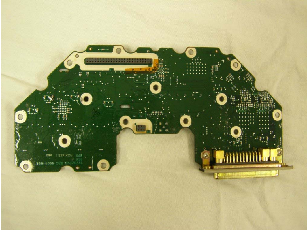
Figure I-11 – Frequency Source - Bottom
