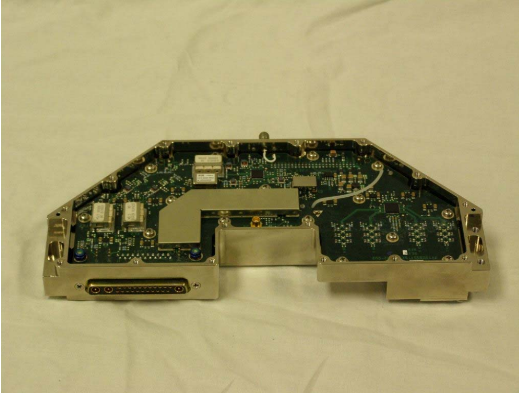
Figure I-3 – Digital Receiver/ Frequency Source Chassis 2
