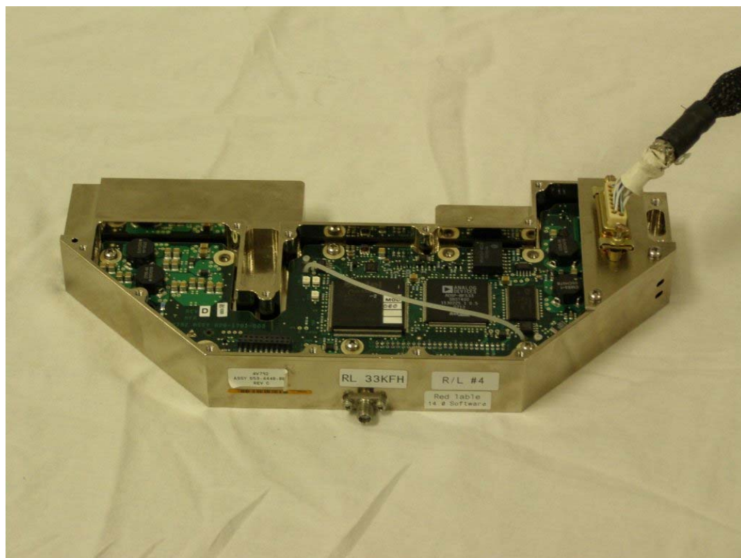
Figure I-2 – Digital Receiver/ Frequency Source Chassis 1
