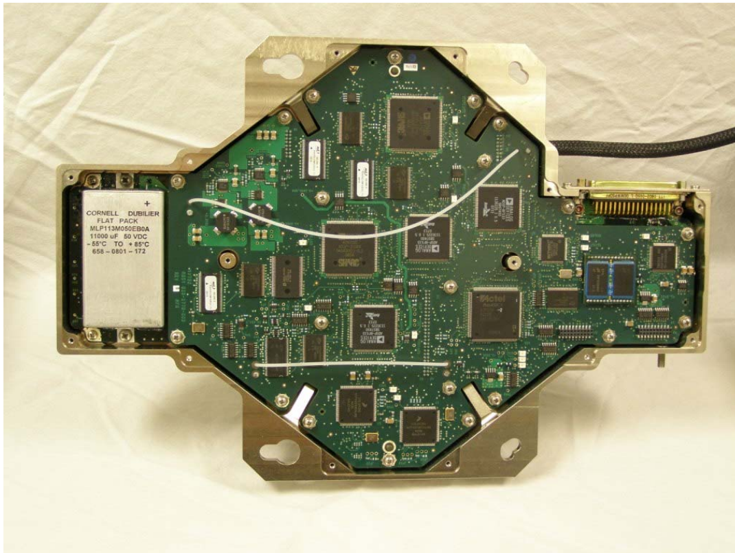
Figure I-1 – Base Assembly View
