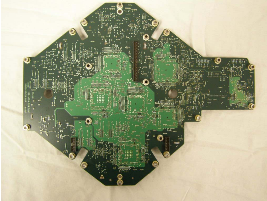
Figure I-5 – System Processor - Bottom
