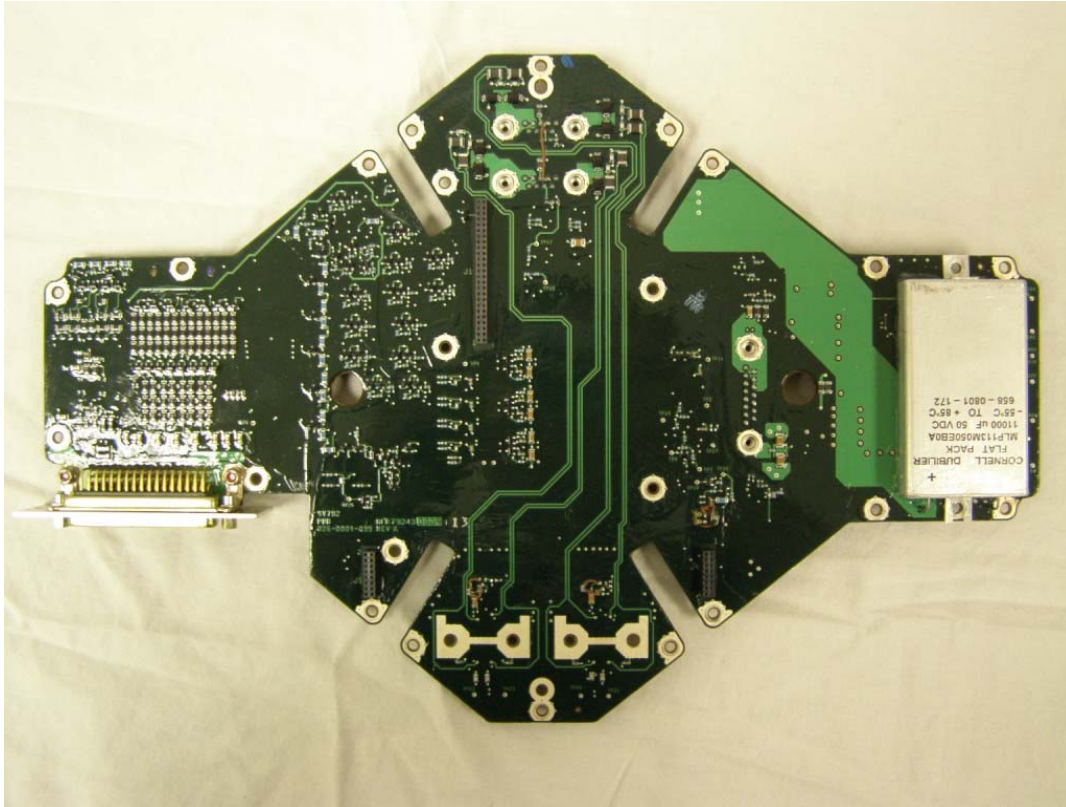
Figure I-7 – Power Supply - Bottom
