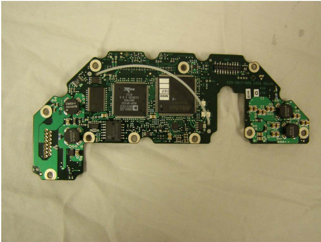
Figure I-8 – Digital Receiver - Top
