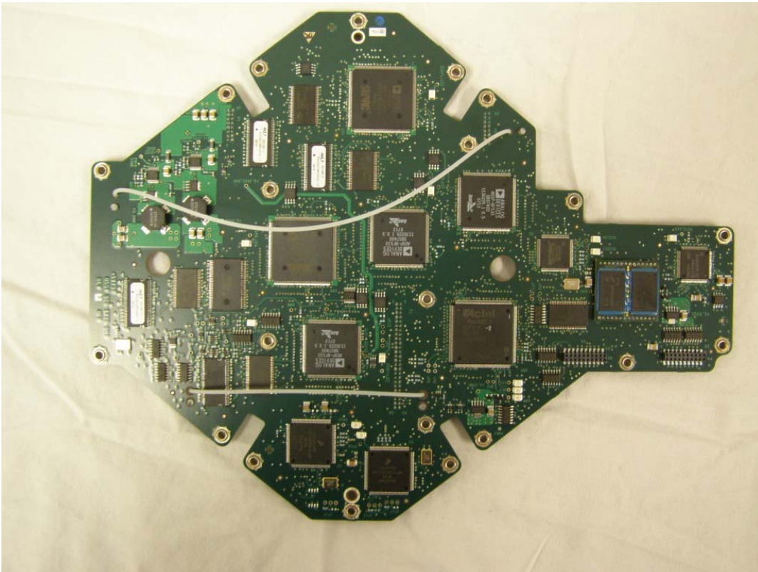
Figure I-4 – System Processor - Top
